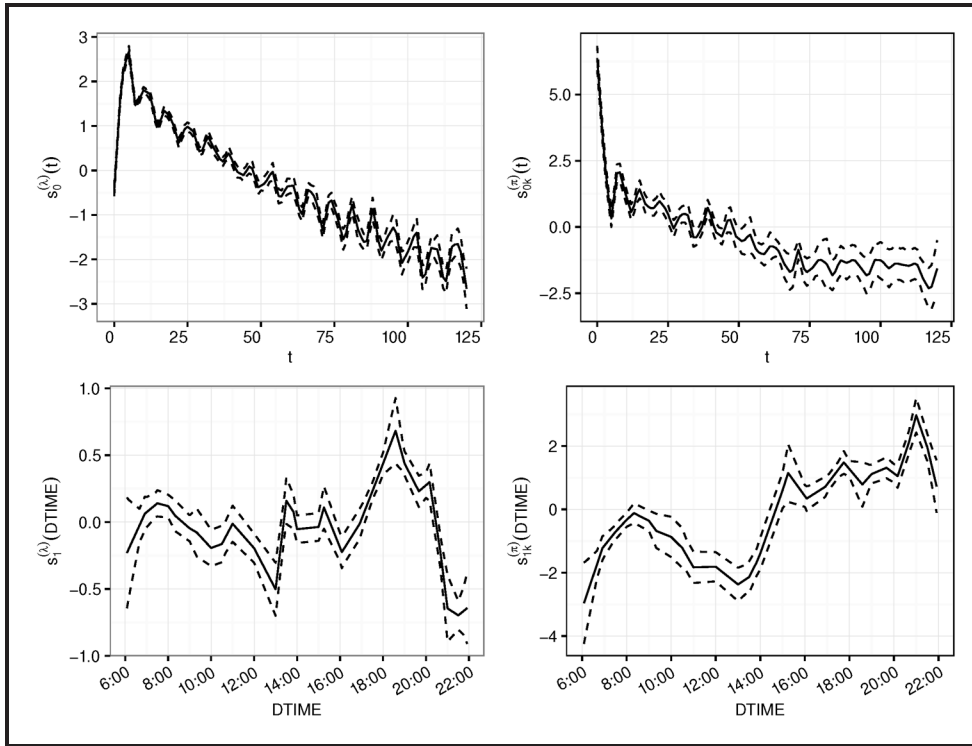
Figure 4 For K = 5 segments, the left-hand panels provide the function estimates for s_0^{(\lambda)}(t) and s_1^{(\lambda)}(DTIME) in Equation (3.2) for bookings on flights that depart on Thursday. The right-hand side shows the estimates of s_{0,k}^{(\pi)}(t) and s_{1,k}^{(\pi)}(DTIME) , k = 1, \dots, 4 in Equation (3.4). The first-stage residuals \hat{\xi} are included (i.e. Model II). The estimates are given by the solid line, while the dashed lines are 99% local confidence bands
