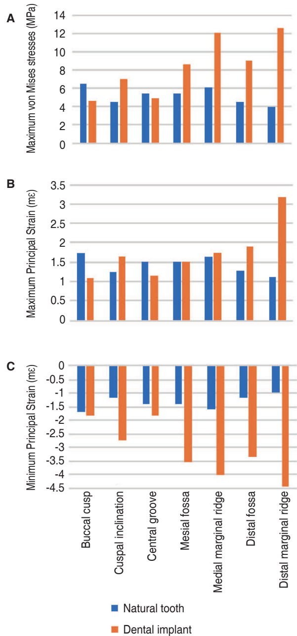
Fig. 5. Maximum von Mises stresses (A), maximum principal strains (B) and minimum principal strains (C) predicted at the mandible for the natural tooth and dental implant assembly. Data are shown for occlusal loading applied at the mesial fossa, distal fossa, buccal cusp, central groove, cuspal inclination, mesial marginal ridge, and distal marginal ridge.
