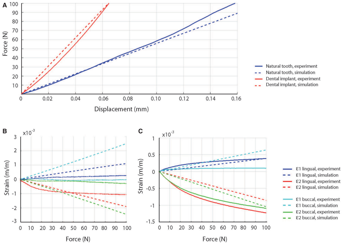
Fig. 3. Force-displacement curves measured experimentally and predicted by the finite element models for the natural and implant tooth assemblies (A), principal strains measured experimentally for the natural tooth on the lingual and buccal sides of the mandible compared to strains calculated using the finite element model (B), and principal strains measured experimentally for the dental implant on the lingual and buccal sides of the mandible compared to strains calculated using the finite element model (C).
