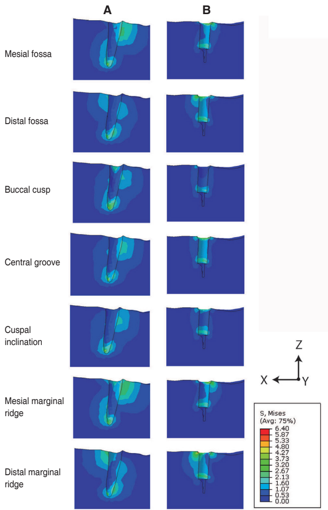
Fig. 4. Contour plots of von Mises stress distributions predicted for the natural tooth (A) and dental implant (B). Data are given for occlusal loading applied at the mesial fossa, distal fossa, buccal cusp, central groove, cuspal inclination, mesial marginal ridge, and distal marginal ridge.
