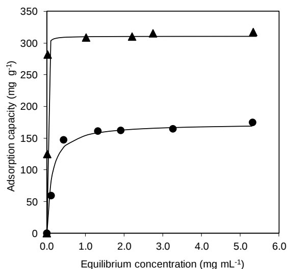
Figure 8. Adsorption isotherms for \alpha -lactalbumin ( \blacktriangle ) and \beta -lactoglobulin ( \bullet ) on the FDU-12-120-NH 2 and the Langmuir equation fits to the experimental data (the solid lines).
