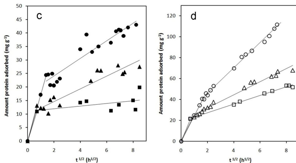
Figure 5. The pseudo-second-order model (a and b) and the intraparticle diffusion model (c and d) plots for adsorption of \beta -lactoglobulin (■: 5 °C, ▲: 15 °C, ●: 25 °C) and \alpha -lactalbumin (□: 5 °C, △: 15 °C, ○: 25 °C) on FDU-12-120.
