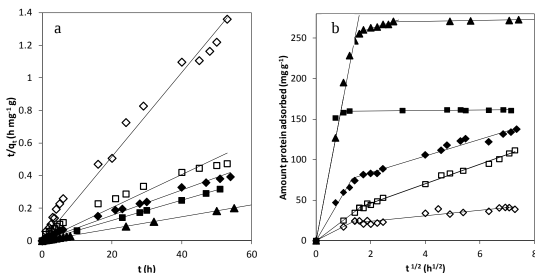
Figure 7. The pseudo-second-order model (a) and the intraparticle diffusion model (b) fitted to the adsorption at 25 °C of \alpha -lactalbumin to the FDU-12-120 ( \square ) and FDU-12-120-NH 2 ( \blacksquare ) and the \beta -lactoglobulin to the FDU-12-120 ( \diamond ) and FDU-12-120-NH 2 ( \blacklozenge ) all at the same initial protein concentration (1.5 mg/mL) and adsorption of \alpha -lactalbumin to the FDU-12-120-NH 2 ( \blacktriangle ) with a higher initial concentration (3 mg/mL).
