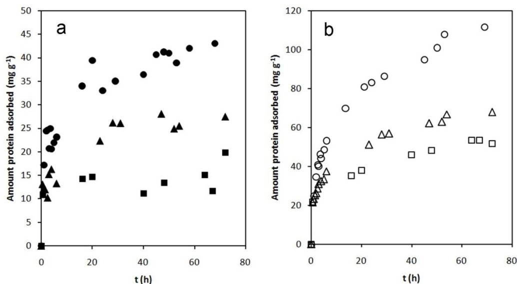
Figure 4. Kinetics of adsorption of a) \beta -lactoglobulin on FDU-12-120 at different temperatures ( \blacksquare : 5 °C, \blacktriangle : 15 °C, \bullet : 25 °C); and b) \alpha -lactalbumin on FDU-12-120 at different temperatures ( \square : 5 °C, \triangle : 15 °C, \circ : 25 °C)
