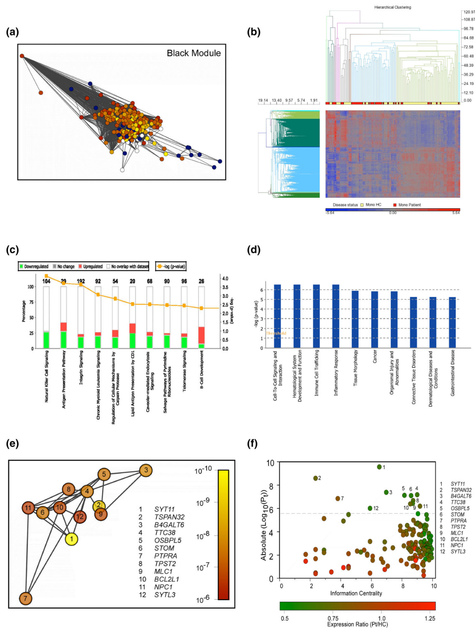
Figure 2. BLACK module gene expression in monocytes. (a) Graph of the BLACK module isolated from the rest of the network, with heat map applied (dark blue represents an uncorrected P -value > 0.05 ; white, an uncorrected P -value < 1.5 \times 10^{-6} , a threshold determined by a conservative Bonferroni correction). (b) Heat map and hierarchical clustering of monocyte differential expression between patients (yellow) and HCs (red) generally grouped patients with RRMS as distinct from HCs in relative gene expression. (c) The top 10 canonical pathways identified by Ingenuity Pathways Analysis (IPA; Ingenuity Systems Inc) for the BLACK module genes expressed in monocytes. Green, downregulated; red, upregulated; and gray, no change. (d) The top 10 enriched pathways identified for the monocyte differential expression analysis (Partek Flow analysis of variance (Partek SG, Singapore)). (e) Graph of the HDE transcripts from the BLACK module with a separate heat map illustrating t -test-derived P -values derived by comparing expression levels of each transcript from monocytes of patients with MS and HCs. Sliding scale representing the least HDE transcripts with P -value of 10^{-6} to most HDE in light yellow with P -value of 10^{-10} , with the threshold determined by a conservative Bonferroni correction. The key identifies the gene symbols associated with each transcript. (f) Dot plot of all transcripts in the BLACK module for each transcript showing the network information score ( x -axis), absolute \log_{10} of the P -value ( y -axis) and differential expression (expression ratio patients/HCs; sliding scale: green represents the most downregulated and red the most upregulated). HC, healthy control; HDE, highly differentially expressed; MS, multiple sclerosis; RRMS, relapsing-remitting multiple sclerosis.
