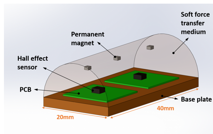
Figure 2. A specific design of the soft tactile sensor with three permanent magnets and two Hall effect sensors embedded inside a semi-cylinder force transfer medium made of Polyurethane (VytaFlex 20).
