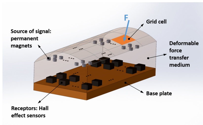
Figure 1. The general case configuration of the proposed tactile sensor with n permanent magnets as the sources of the signal and m Hall effect sensors as the signal receptors, embedded in the deformable force transfer medium. The intended spatial resolutions of the contact point localisation procedure are defined by the size of the grid cell.
