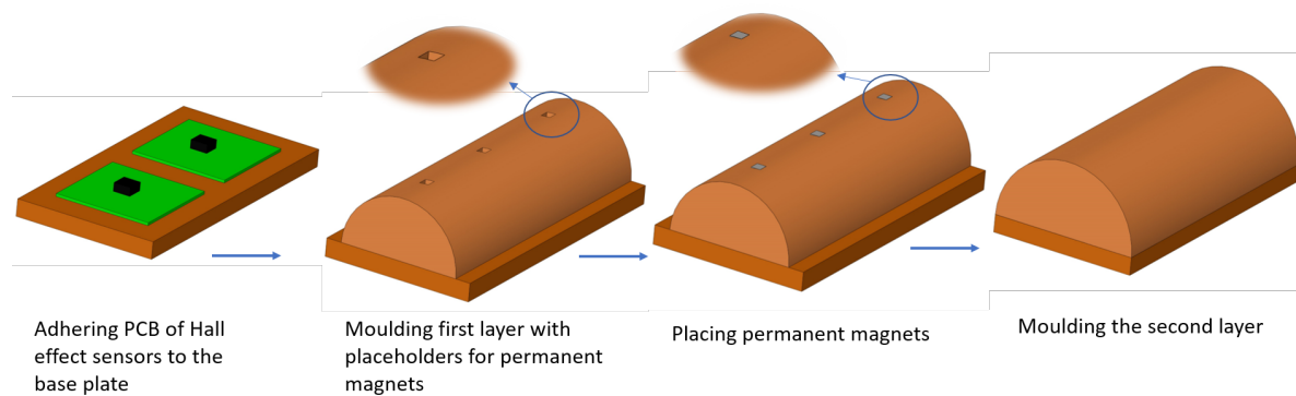
Figure 3. Sensor fabrication procedure.
