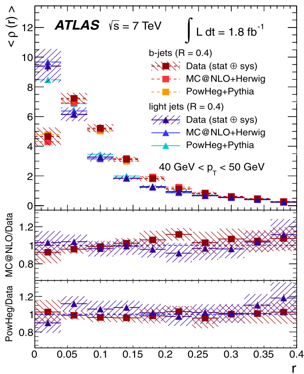
Fig. 14 Differential jet shapes \langle\rho(r)\rangle as a function of the radius r for light jets (triangles) and b -jets (squares). The data are compared to MC@NLO+HERWIG and POWHEG+PYTHIA event generators for 40\text{ GeV} < p_T < 50\text{ GeV} . The uncertainties shown include statistical and systematic sources, added in quadrature
