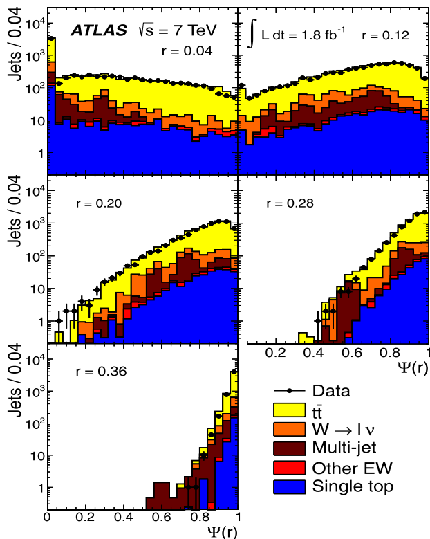
Fig. 7 Distribution of R = 0.4 light jets in the single-lepton channel as a function of the integrated jet shapes \Psi(r) for different values of r
