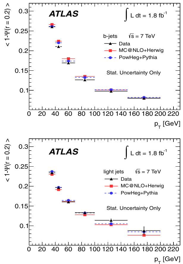
Fig. 8 Dependence of the b -jet ( top ) and light-jet ( bottom ) shapes on the jet transverse momentum. This dependence is quantified by plotting the mean value \langle 1 - \Psi(r = 0.2) \rangle (the fraction of energy in the outer half of the jet cone) as a function of p_T for jets in the single-lepton sample
