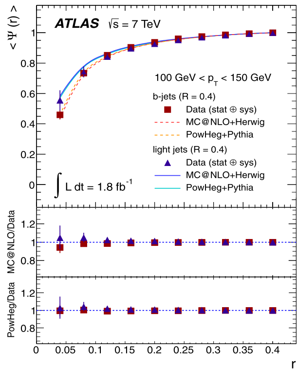
Fig. 21 Integrated jet shapes \langle\Psi(r)\rangle as a function of the radius r for light jets (triangles) and b -jets (squares). The data are compared to MC@NLO+HERWIG and POWHEG+PYTHIA event generators for 100\text{ GeV} < p_T < 150\text{ GeV} . The uncertainties shown include statistical and systematic sources, added in quadrature
