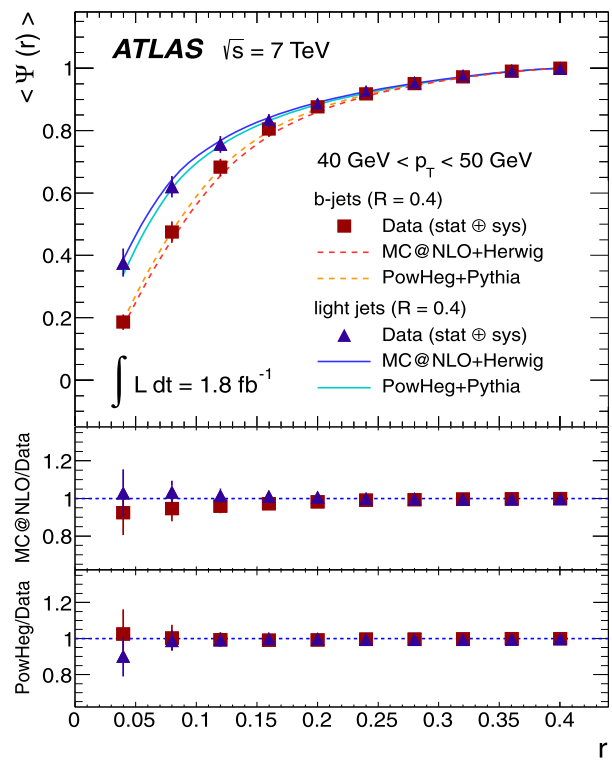
Fig. 15 Integrated jet shapes \langle\Psi(r)\rangle as a function of the radius r for light jets (triangles) and b -jets (squares). The data are compared to MC@NLO+HERWIG and POWHEG+PYTHIA event generators for 40\text{ GeV} < p_T < 50\text{ GeV} . The uncertainties shown include statistical and systematic sources, added in quadrature
