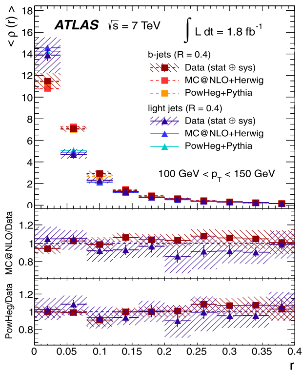
Fig. 20 Differential jet shapes \langle\rho(r)\rangle as a function of the radius r for light jets (triangles) and b -jets (squares). The data are compared to MC@NLO+HERWIG and POWHEG+PYTHIA event generators for 100\text{ GeV} < p_T < 150\text{ GeV} . The uncertainties shown include statistical and systematic sources, added in quadrature
