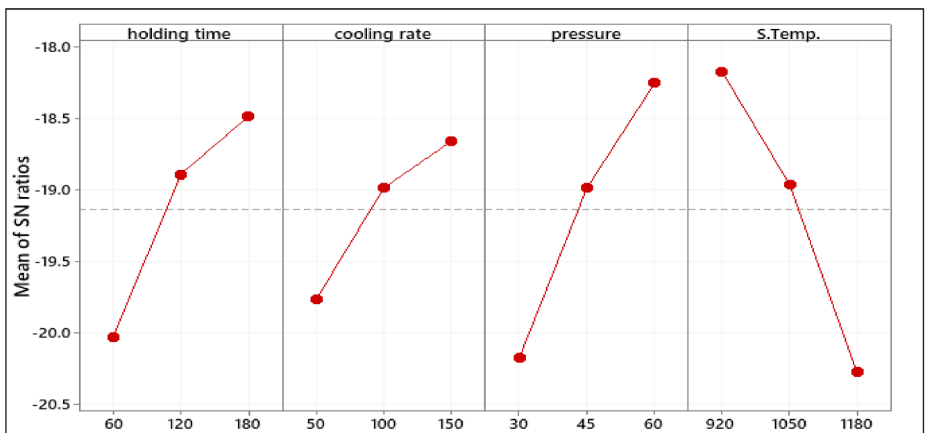
Figure 6. Mean S/N ratio of Mr^{\perp} .
