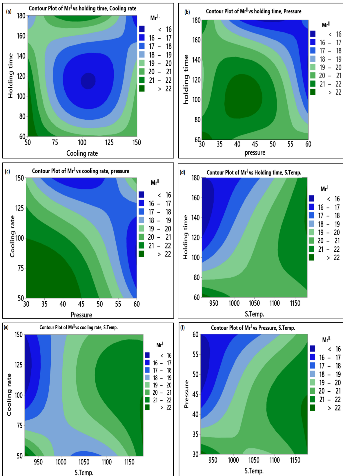
Figure 10. Contour plot for Mr^{II} : (a) Holding time vs. cooling rate; (b) Holding time vs. pressure; (c) Cooling rate vs. pressure; (d) Holding time vs. S. temp.; (e) Cooling rate vs. S. temp.; (f) Pressure vs. S. temp.
