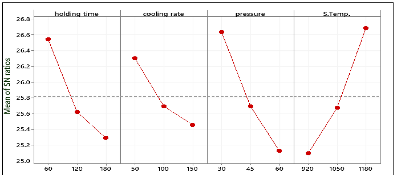
Figure 5. Mean S/N ratio of Mr^{\parallel} .
