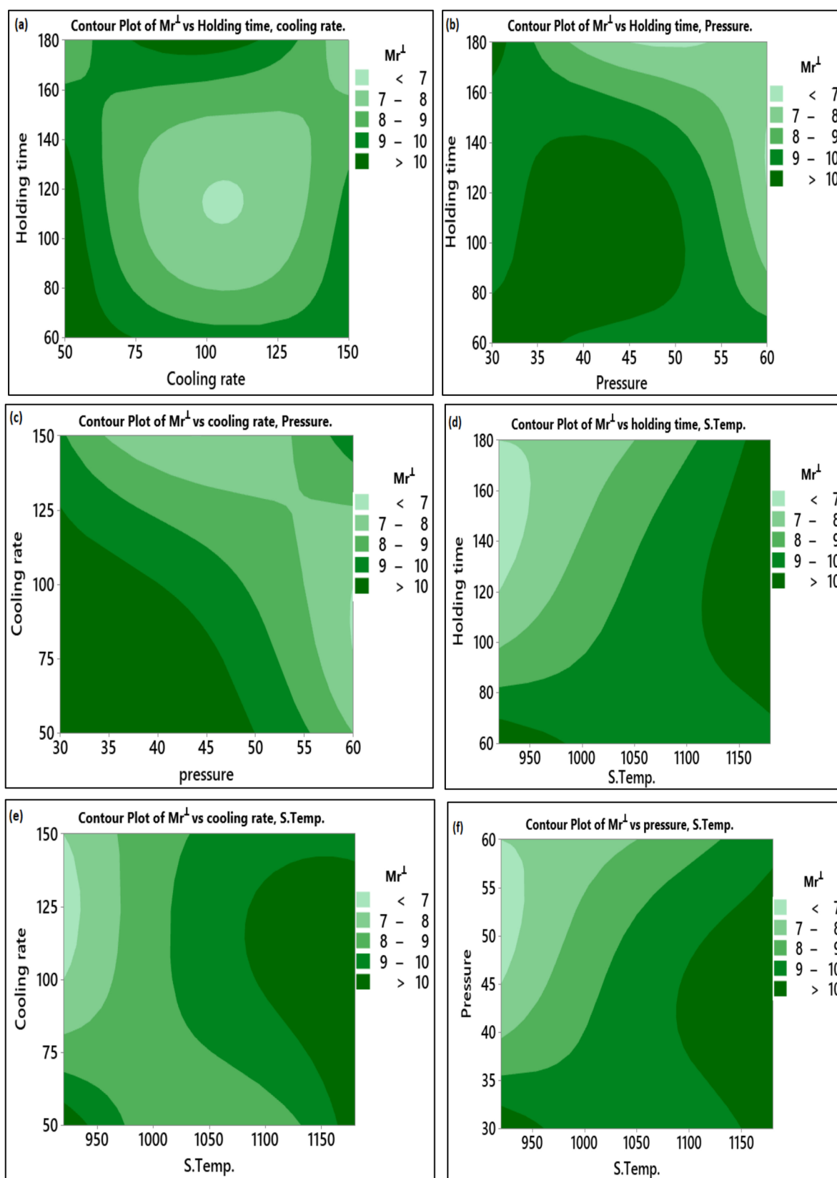
Figure 11. Contour plot for Mr^L : (a) Holding time vs. cooling rate; (b) Holding time vs. pressure; (c) Cooling rate vs. pressure; (d) Holding time vs. S. temp.; (e) Cooling rate vs. S. temp.; (f) Pressure vs. S. temp.
