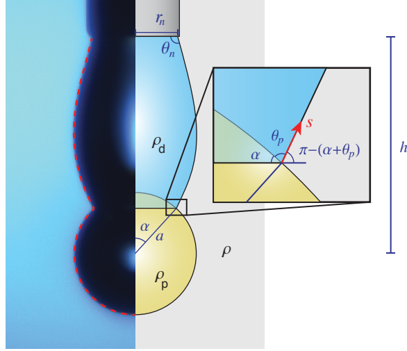
Figure 1: Gravitational forces on both the particle and the liquid drop result in coupled drop deformations of a compound pendant drop. Right side: A schematic representation of a spherical particle attached to the interface of an axisymmetric pendant drop emerging from a needle into a bulk fluid phase. Left side: An image of a compound pendant drop from Fig. 2 a (v) with the drop shape (red dashed line) found by solving the Young-Laplace equation to determine the drop and particle Bond numbers.
