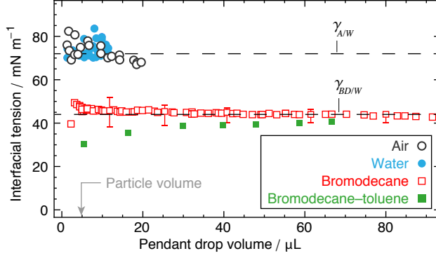
Figure 4: The interfacial tension for each of the four particle-drop systems deduced by compound pendant drop tensiometry shown in Fig. 2: the air-water interfacial tension calculated from a water drop in air (filled blue circles) and from an air bubble in water (open white circles); a bromodecane drop in water (open red squares) and a bromodecane-toluene drop density matched to water (solid green squares) demonstrates the applicability of the method even at zero Bond number.
