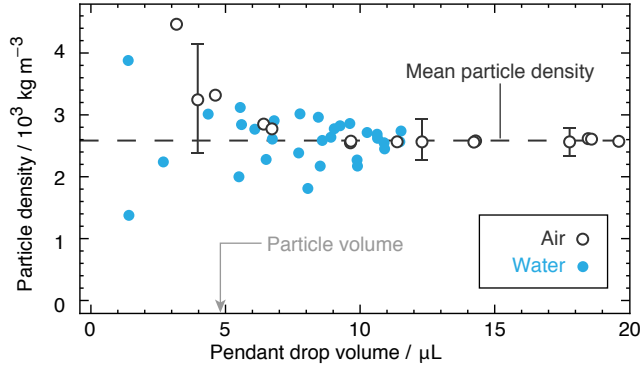
Figure 3: The density of the silica particle deduced from the compound pendant water drop in air (filled blue circles) and the compound pendant bubble in water (open white circles) experiments. The mean density calculated by independently weighing the particles with a microbalance is shown as the dashed line. Representative experimental uncertainties are included.
