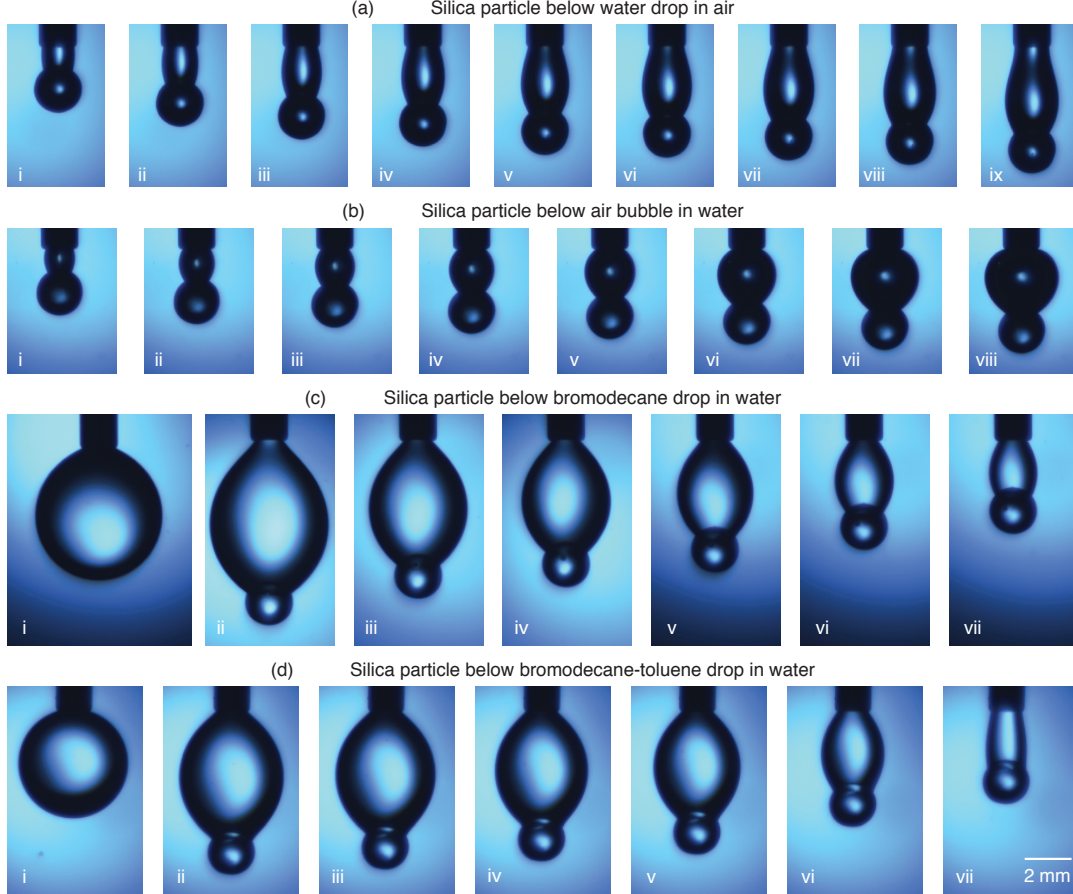
Figure 2: (a) A silica particle attached to a pendant water drop in air: (i)-(ix) Gravitational force on the drop and particle elongates the drop as the drop volume increases. (b) A silica particle attached to a pendant air bubble in water: (i)-(viii) Variation of the bubble shape as the volume is increased by injecting air via the needle. The drop Bond number Bo_d \sim -1 , so the buoyancy forces on the bubble and the particle act in opposite directions. (c) Bromodecane pendant drop in water with drop Bond number Bo_d \sim 0.005 : (i) a near spherical drop shape prior to particle attachment, (ii)-(vii) drop shape after attachment of a silica particle at decreasing drop volume. (d) Density matched bromodecane-toluene pendant drop in water with zero drop Bond number Bo_d = 0 : (i) a spherical drop prior to particle attachment, (ii)-(vii) drop shape after attachment of a silica particle at decreasing drop volume. The scale bar shown applies to all images.
