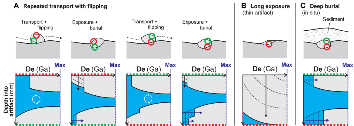
Fig. 6. Additional and more complex pathways of rock artifacts in the landscapes and the corresponding luminescence signal (note that all pathways continue from a semi-embedded artifact as shown in Fig. 3C). (A) Repeated transport with artifact flipping and subsequent shielding, (B) the case of a thin artifact subject to complete bleaching from the exposed surface, and (C) shielding by deep in situ burial (e.g., via aeolian deposition).
