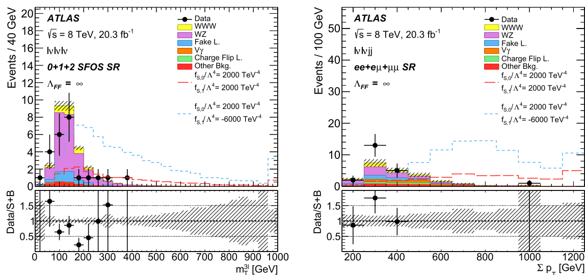
Fig. 3 The distribution of m_T^{3\ell} for the \ell\nu\ell\nu\ell\nu channel (left) and the distribution of \Sigma_{PT} for the \ell\nu\ell\nu jj channel (right) as observed in the data (dots with error bars indicating the statistical uncertainties) and as expected from SM signal and background processes. The ratios between the observed numbers of events in data and the expected SM signal plus background contributions are shown in the lower panels. The hashed bands results from the systematic uncertainties on the
