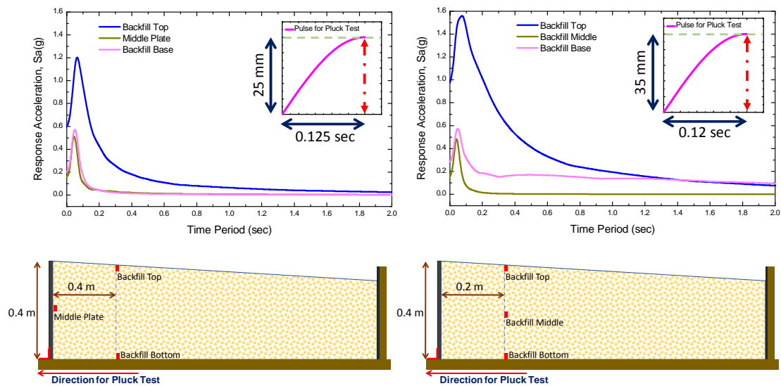
Figure 6 Horizontal spectral acceleration for 25mm and 35 mm amplitude pluck test.
