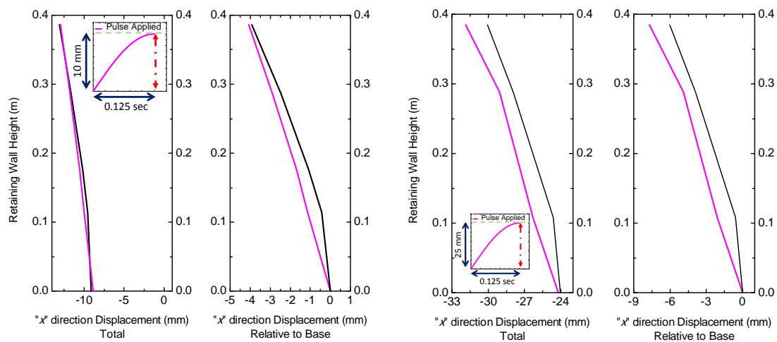
(a) “x” direction displacement along the wall height (bottom to top) for 10 mm amplitude pluck test. (b) “x” direction displacement along the wall height (bottom to top) for 25 mm amplitude pluck test.
