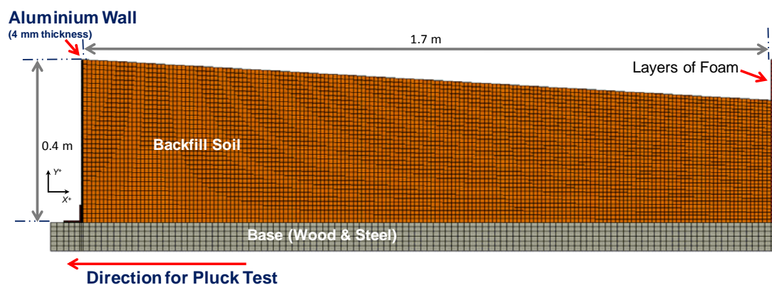
Figure 4 FE model of retaining wall in Abaqus.
