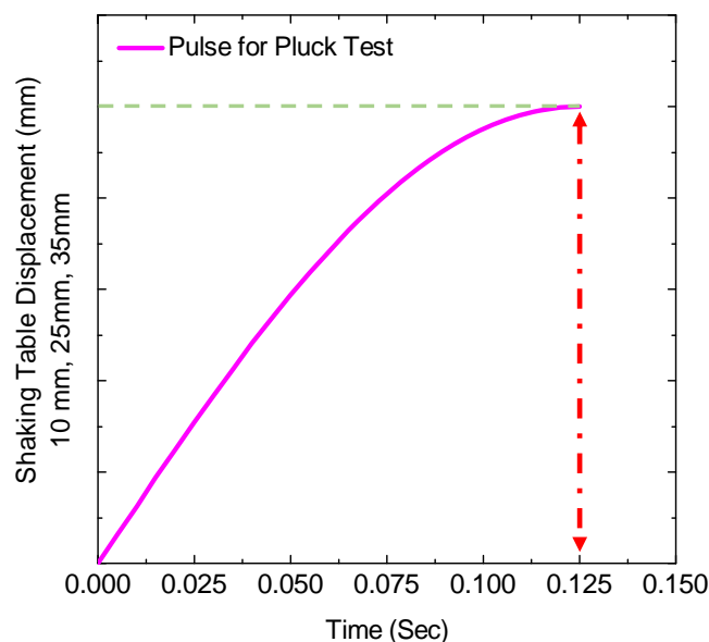
Figure 3 Pulse used for pluck test.
