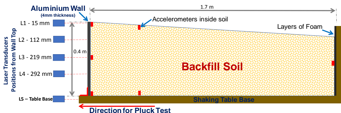
Figure 1 Details of scaled down retaining wall model.
