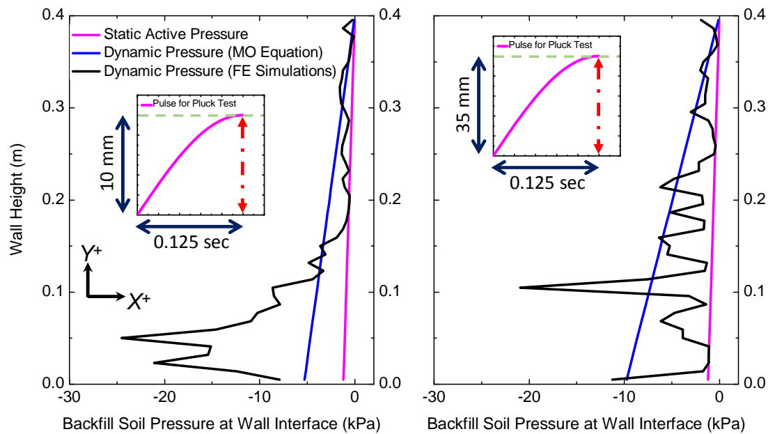
Figure 7 Backfill soil pressure behind the retaining wall.
