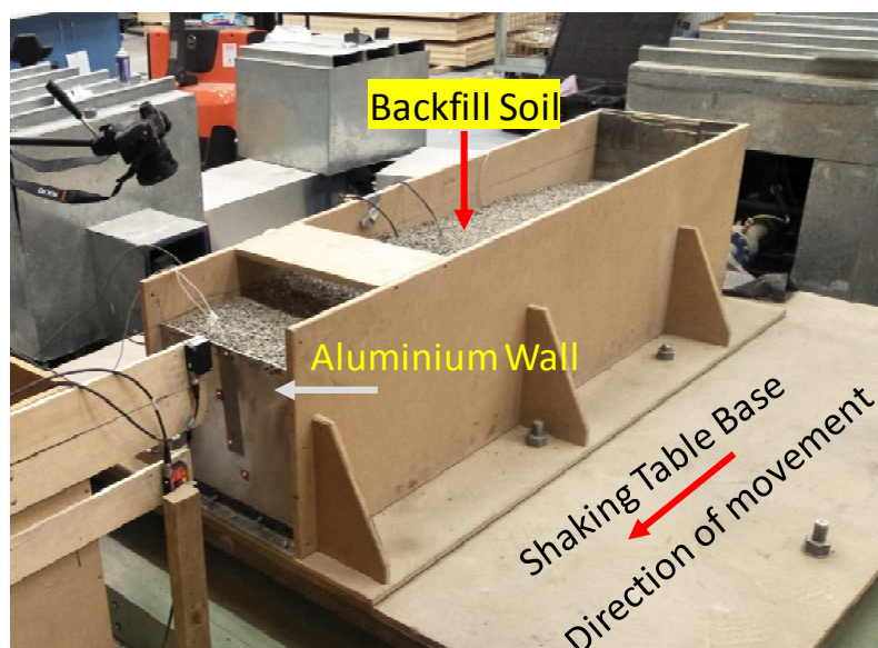
Figure 2 Experimental setup at The University of Melbourne.
