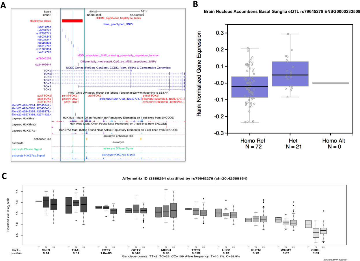
Figure 2. Functional prediction of the hit haplotype block. (A) Functional annotation of the hit haplotype block. The hit haplotype block (red bar on the left top showing the block and blue bars showing the genotype single nucleotide polymorphisms [SNPs] in Generation Scotland: The Scottish Family Health Study [GS:SFHS]) is located in the intron region and a proportion of an adjacent exon of gene TOX2 , overlapped with Fantom5 enhancers and transcription start sites, and regulatory-relevant histone modification peaks (H3K27Ac and H3K4Me1). Within the block, 38 imputed SNPs were associated with major depressive disorder (MDD), using SNP rs79645278 (pink) as an example. This SNP is located in the peak of active enhancer in astrocyte (highlighted with blue line). (B, C) Boxplots showing tissue-specific effect from SNPs that are both associated with MDD in GS:SFHS and gene expression, using SNP rs79645278 as an example. (B) The minor allele of rs79645278 upregulates the expression of a long noncoding RNA RP1-269M15.3 in the tissue nucleus accumbens basal ganglia. (C) The minor allele of rs79645278 upregulates the expression of gene TOX2 in the frontal cortex (FCTX). CRBL, cerebellar cortex; eQTL, expression quantitative trait loci; HIPPO, hippocampus; MEDU, medulla (specifically inferior olivary nucleus); OCTX, occipital cortex (specifically primary visual cortex); PUTM, putamen; SNIG, substantia nigra; THAL, thalamus; TCTX, temporal cortex; WHMT, intralobular white matter.
