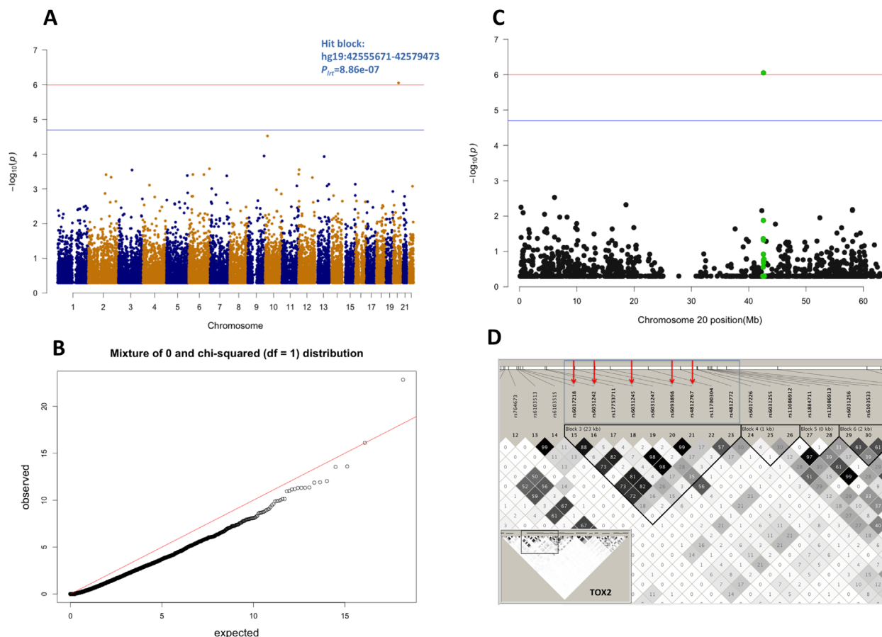
Figure 1. Genome-wide haplotype-block-based regional heritability mapping results on major depressive disorder in Generation Scotland: The Scottish Family Health Study (GS:SFHS). (A) Manhattan plot. Each point represents a haplotype block. The location of the point is the mid-position of the haplotype block. (B) A quantile-quantile plot for the likelihood ratio test (LRT). The LRT statistics are distributed as a mixture of 0 and chi-squared ( df = 1 ) distribution. (C) Zoom-in region of the hit haplotype block region in chromosome 20. (D) Linkage disequilibrium (LD) structure within the hit haplotype block in GS:SFHS. The block is located in gene TOX2 ; it contains nine genotyped common SNPs (blue boxes), and five of them are in high LD (red arrows) in GS:SFHS.
