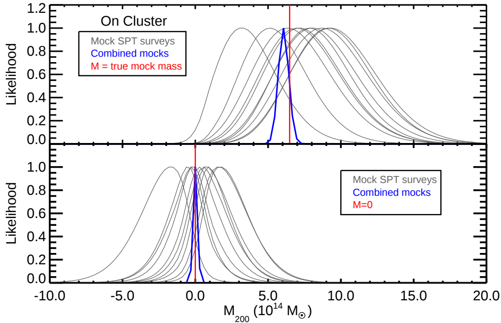
FIG. 1.— Constraints on M_{200} from the analysis of mock data that is designed to mimic real data from the SPT. The top panel shows the likelihood as a function of M_{200} for patches centered on clusters; the bottom panel shows the same for patches centered at random points ( off-cluster ). Each gray curve represents the constraint obtained from a single realization of an SPT-like survey that detects 513 clusters; the blue curves are combined constraints from 50 such realizations.
