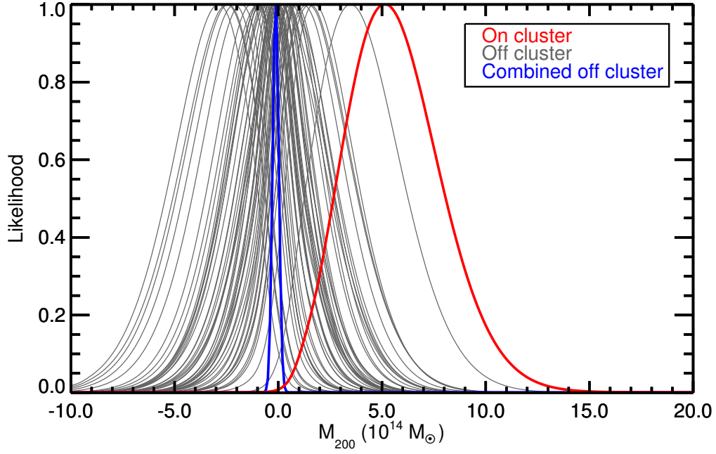
FIG. 2.— Constraints on M_{200} resulting from analysis of SPT data. The thick red curve is our result for 513 on-cluster cutouts, while each thin gray curve is our result for a separate realization of 513 off-cluster cutouts. The combined constraint from the 50 sets of off-cluster cutouts is the thick blue curve.
