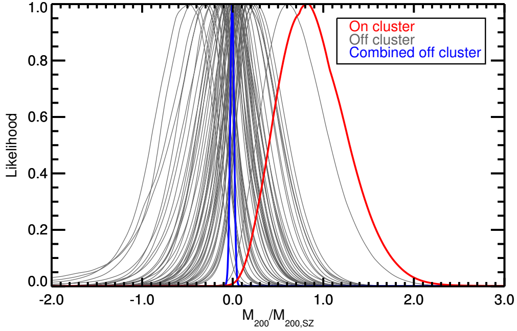
FIG. 3.— Same as Fig. 2 except the likelihood has been computed as a function of M_{200}/M_{200,SZ} , where M_{200,SZ} is the cluster mass computed from the measured tSZ signal as described in Bleem et al. (2015).
