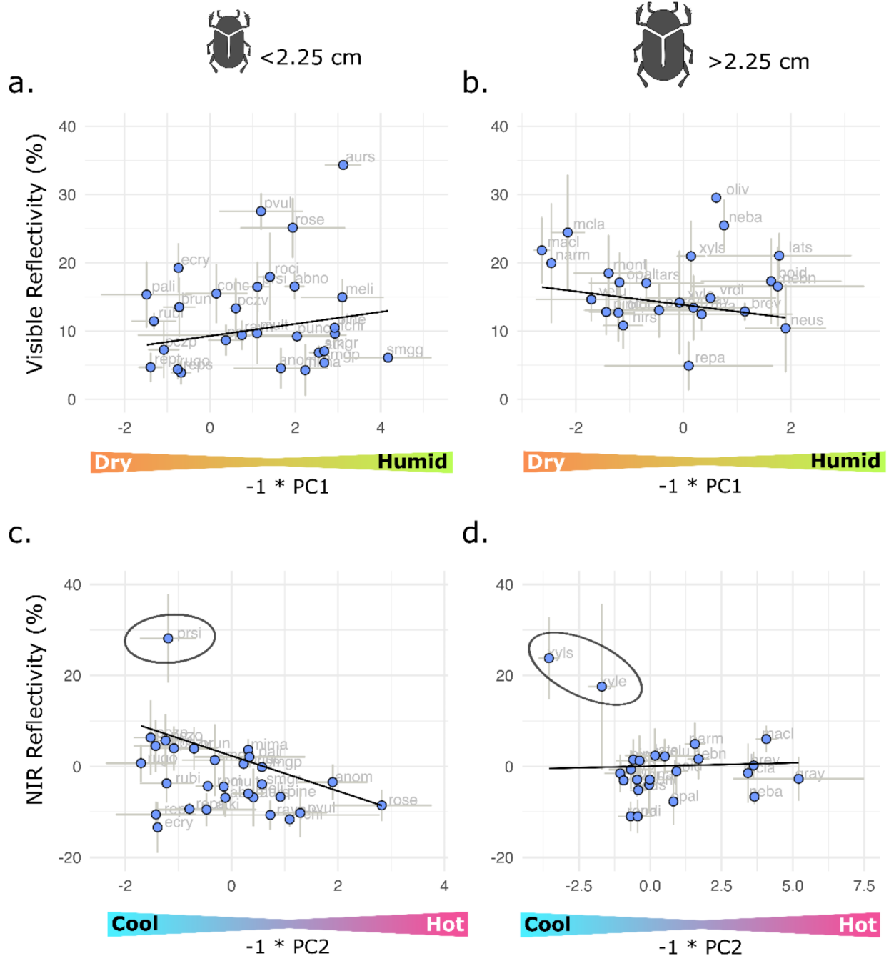
Fig. 3. Effects of the interactions between climate and size on reflectivity. Trend lines were calculated based on the estimates of the PGLS models but only the correlations with p -value < 0.05 in the MCC tree are shown (Supplementary 6). The negative of the principal components is plotted for easier interpretation. PC2 was fixed at the mean value for all beetles in (a) and (b) while PC1 was fixed at the mean value for all beetles in (c) and (d). For visualization, species are divided into those smaller and larger than the mean body size (2.25 cm). The plots show the mean and standard deviation (error bars) of the studied optical properties and PC values per species. NIR reflectivity is given as the residuals of a simple linear model with visible reflectivity as a predictor for visualization purposes. PGLS analyses excluding the species circled in (c) and (d) did not show any correlation between temperature and NIR reflectivity (Supplementary Table S5 and S6).
