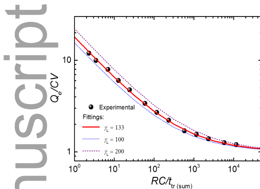
Figure 5. Extracted charge normalized to the amount of charge on the electrodes ( CV ) versus the faster carrier transit time normalized to the RC -time. The photovoltage transients (devices similar to Figure 1 ) are measured at high laser fluences that saturate the photovoltage (number of photons \gg CV/e ) and subsequently integrated to obtain the extracted charge. The experimental results are in agreement with the results from injection based methods [ Equation (7) ], i.e. , \gamma_L = 133 . The dashed purple and dotted blue lines correspond to non-matching fittings in order to show the sensitivity of the fittings to the \gamma value.
