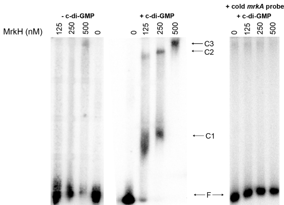
Figure 9. Analysis of the binding of MrkH-8×His to the mrkA regulatory region by EMSA. The ^{32} P-labelled PCR fragment containing the mrkA regulatory region was generated using primer pairs ^{32} P-Px1mrkARev and mrk295F. The mrkA fragment was mixed with varying amounts of the purified MrkH-8×His protein (from 0 to 500 nM) in the absence or presence of c-di-GMP (200 \mu M). Following incubation at 30°C for 20 min, the samples were analyzed on native polyacrylamide gels. The right-hand panel shows control reactions with approximately 100-fold molar excess of the unlabeled (cold) mrkA promoter fragment (specific competitor DNA), used to demonstrate the specificity of the c-di-GMP-mediated MrkH binding to the mrkA promoter region. The unbound DNA (F) and protein-DNA complexes (C1, C2 and C3) are marked.
