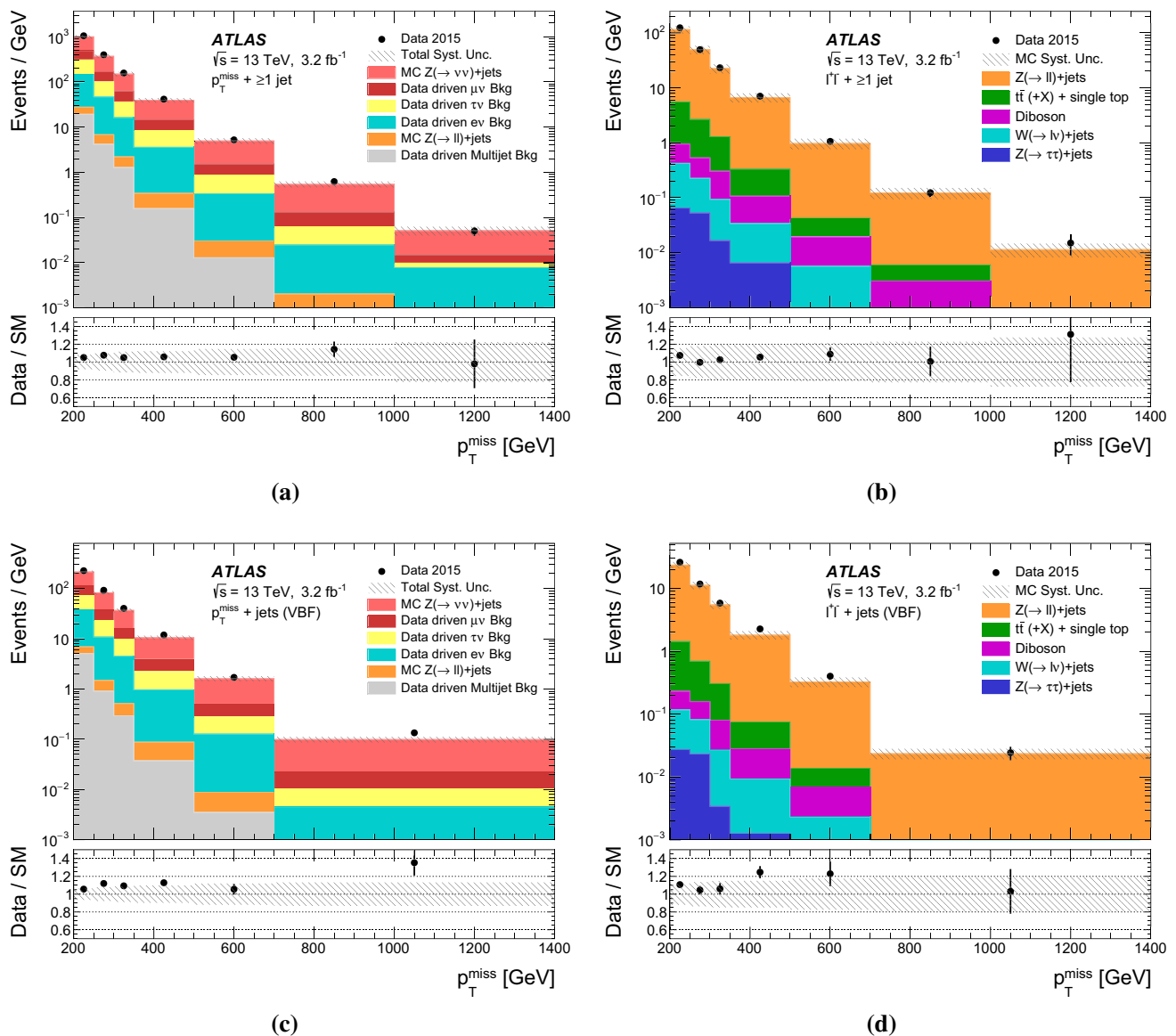
Fig. 2 Comparisons between detector-level distributions for data and MC simulation of Z \rightarrow \nu\bar{\nu} and Z \rightarrow \ell\ell events plus predicted backgrounds in selected a , c p_T^{\text{miss}} + \text{jets} events and b , d \ell^+\ell^- + \text{jets} events as a function of the p_T^{\text{miss}} variable in the a , b \geq 1 jet phase space and c , d VBF phase space. The lower panel shows the ratio of data to the Standard Model prediction. The error bars show the statistical
