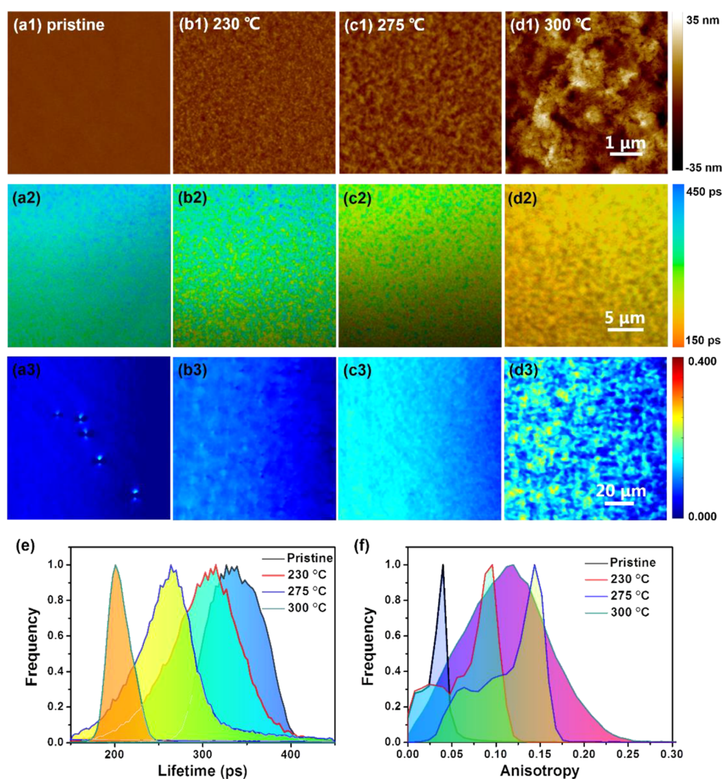
Figure 3. Atomic force microscopy (AFM) images of PODPF films (a) before annealing and after annealing at (b) 230, (c) 275, and (d) 300 °C; the size of the AFM images is 5 \mu\text{m} \times 5 \mu\text{m} . (a2–d2) FLIM and (a3–d3) FAIM images of corresponding films. (e) Average fluorescence lifetime and (f) fluorescence anisotropy distribution histograms of PODPF films following annealing at different temperatures. All film thickness are about 105–110 nm.
