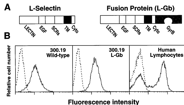
Figure 1. Generation of L-selectin-expressing cell lines. (A) Structure of L-selectin and the L-selectin-GyrB (L-Gb) fusion protein containing the entire L-selectin protein in-frame with the \text{NH}_2 -terminal 24-kD subdomain of the B subunit of bacterial DNA gyrase (GyrB). Domains: EGF, epidermal growth factor-like; SCR, short consensus repeat; TM, transmembrane; Cyto, cytoplasmic. (B) Cell-surface expression of wild-type L-selectin or L-Gb in stably-transfected 300.19 cells and wild-type L-selectin expression by human blood lymphocytes. Cells were isolated and stained with FITC-conjugated LAM1-116 mAb specific for L-selectin (solid line) or an isotype-matched, nonbinding control mAb (dashed line) as previously described (16). Fluorescence histograms from flow cytometry analysis are on a three-decade log scale and are representative of results from at least five experiments.
