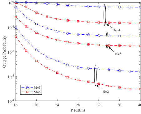
Fig. 5: Outage probability for multi-user networks with N = 2, 3, 4 , M = 5, 6 , L = 20 and D_L = 10 km
