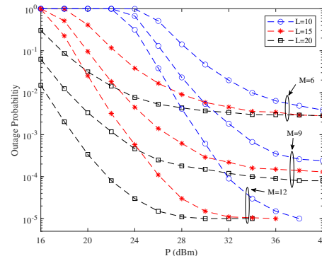
Fig. 4: Outage probability for two-user networks with M = 6, 9, 12, L = 10, 15, 20 and D_L = 10 km
