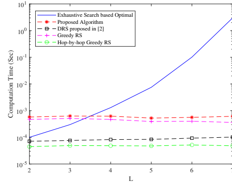
Fig. 3: Average computation time versus L for a two-user network with M = 3 and D_L = 3 km
