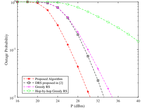
Fig. 2: Outage probability for multi-user network with N = 3, M = 4, L = 6 and D_L = 3 km
