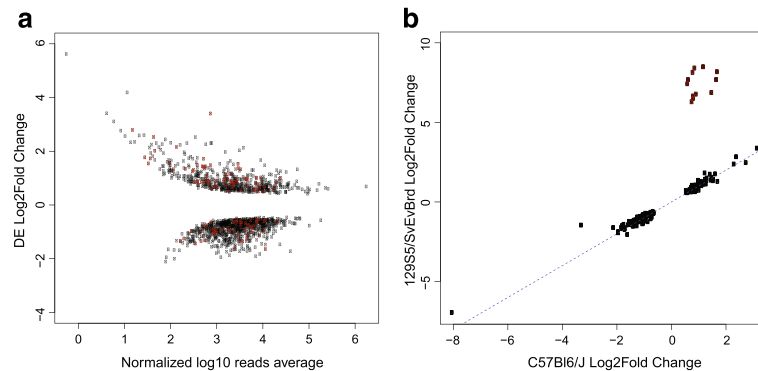
Fig. 6 a log2fold ratios (y axis) and their corresponding average of normalized counts (x axis) for all DE genes between Df/+^{Bl6} and +^{129}/+^{Bl6} MEFs. Positive values indicate higher expression in +^{129}/+^{Bl6} MEFs, while negative values indicate higher expression in Df/+^{Bl6} MEFs. Shown in red are all the DE genes present on chromosome 4. b log2fold ratios for DE 129S5/SvEv Brd alleles (y axis) and DE C57Bl6/J alleles (x axis) in Df/+^{Bl6} MEFs. Notice the high degree of correlation between the allelic log2fold changes when compared to a perfect correlation score (1, blue dashed line). Genes shown in red fall within the deletion sequence, and therefore display a different behavior compared to other alleles
