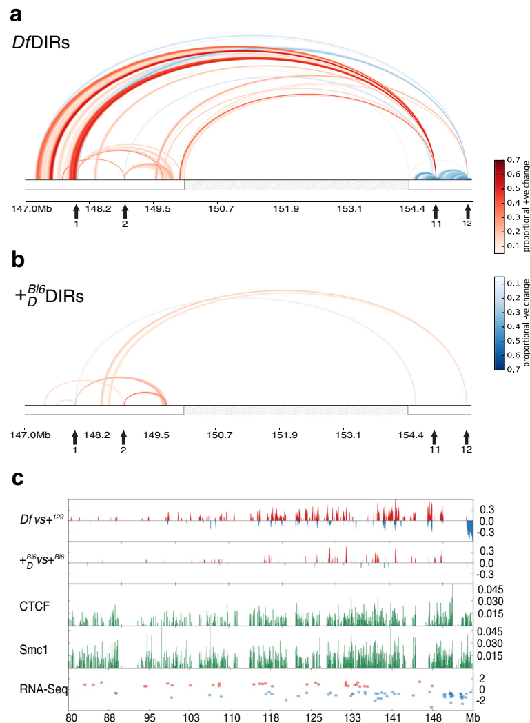
Fig. 3 Df and + Bl6 / D DIRs along chromosome 4. a “Rainbow plot” for the 4E2 region representing the DIRs for the comparison between Df and + 129 , and between + Bl6 / D and + Bl6 computed with a 20 Kb smoothing factor for the viewpoints surrounding the deletion b . Rainbow plots were used to visualize both short and long-range interaction changes. The arcs represent increased interaction probabilities (red) or decreased interaction probabilities (blue), with the strength of signal color coded. For visual clarity we only show signals with strength >10 %, and do not include contacts inside the deletion region for + Bl6 / D in b . Grey arrows annotate positions for viewpoints 1, 2 (upstream of deletion) and 11, 12 (downstream of deletion, towards telomeric end). c Positions of DIRs for all viewpoints 1, 2, 11 and 12 are compared against structural protein binding sites. First track is for Df and + 129 comparisons and second track is for + Bl6 / D and + Bl6 comparison. DIRs with increased/decreased contact probabilities compared to WT are plotted in red/blue. Shown in the third and fourth tracks (green bars) are the running average over 20 Kb window for CTCF and Smc1 binding site footprint, respectively. The fifth track displays fold change for Df /+ Bl6 DE genes, color coded (red, over-expressed in Df /+ Bl6 MEFs; blue, over-expressed in + 129 /+ Bl6 MEFs)
