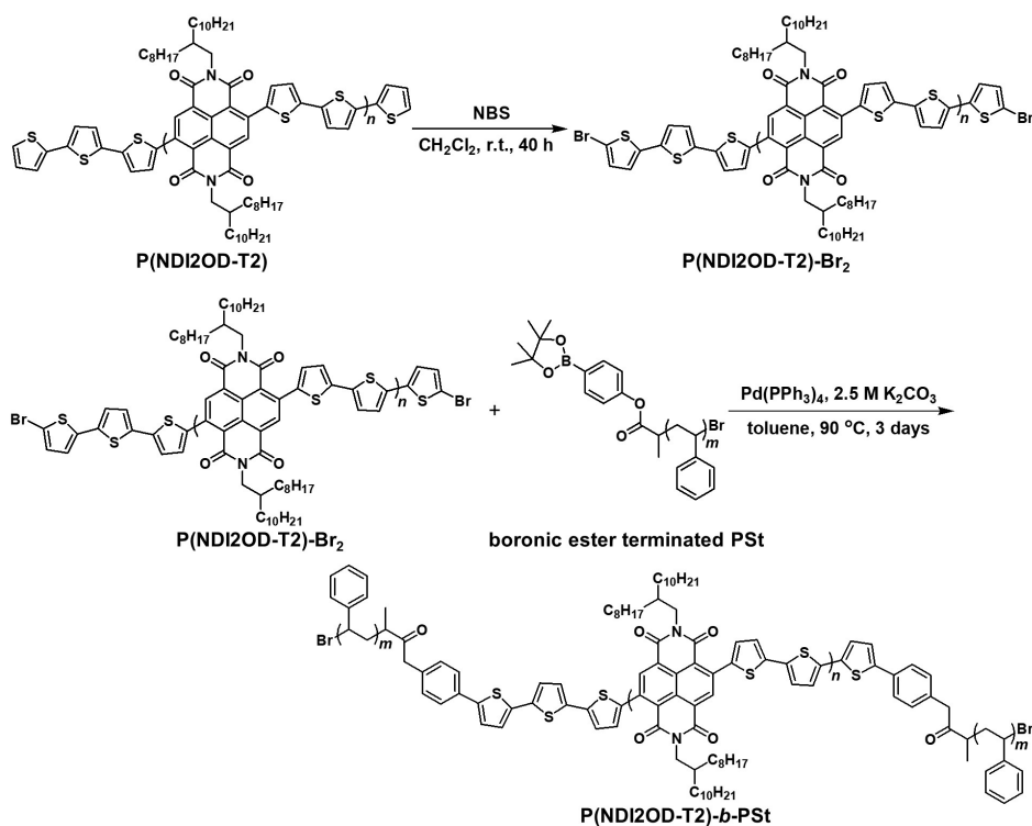
Figure 2. Synthetic scheme of P(NDI2OD-T2)- b -PSt.
