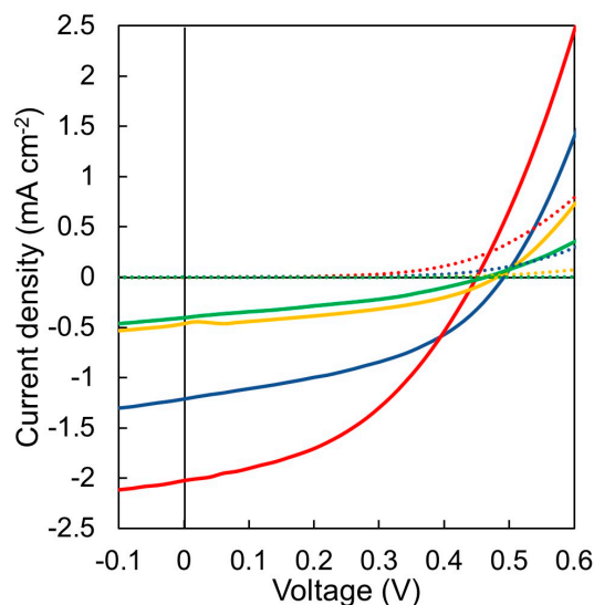
Figure 7. J - V characteristics of P3HT/P(NDI2OD-T2) (blue), P3HT- b -PSt/P(NDI2OD-T2)- b -PSt (red), P3HT- b -PSt/P(NDI2OD-T2) (yellow) and P3HT/P(NDI2OD-T2)- b -PSt (green) exhibiting the best power-conversion efficiency (PCE) of each. Solid and dotted lines represent light and dark conditions, respectively.
