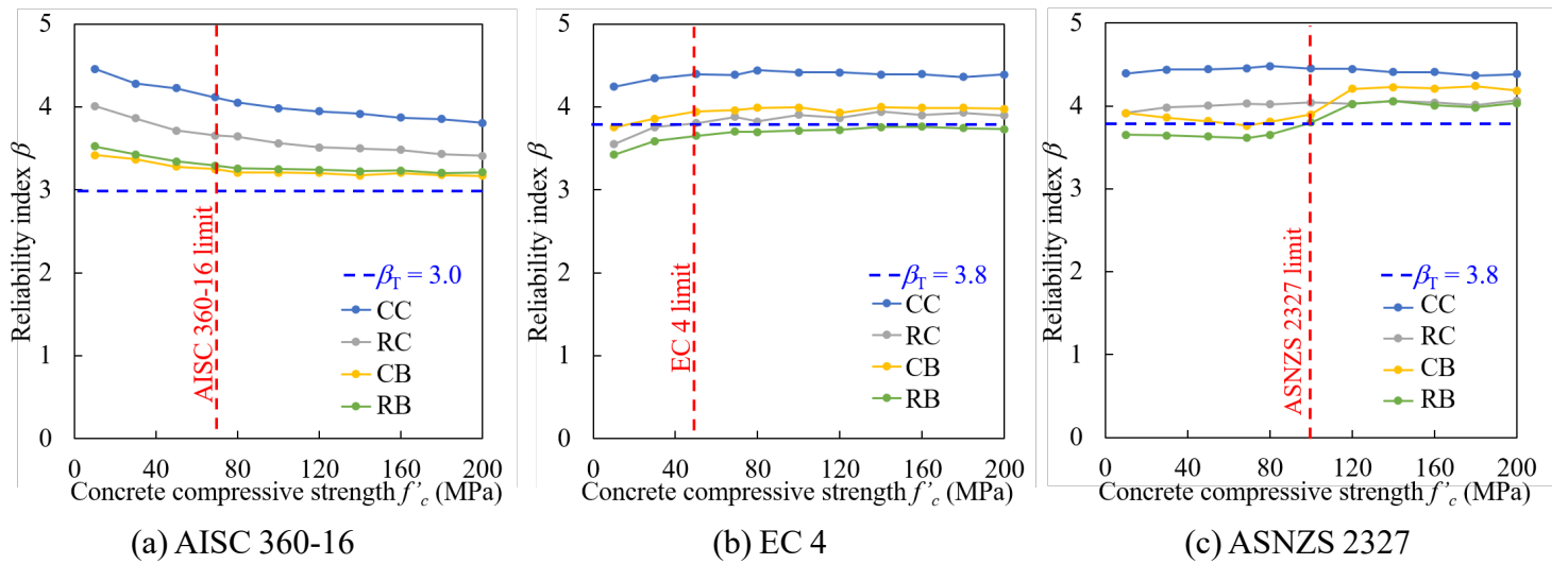
Fig. 15. Effect of f'_c on the reliability index of three codes
