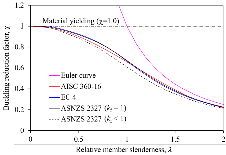
Fig. 5. Column curves from three considered design codes
