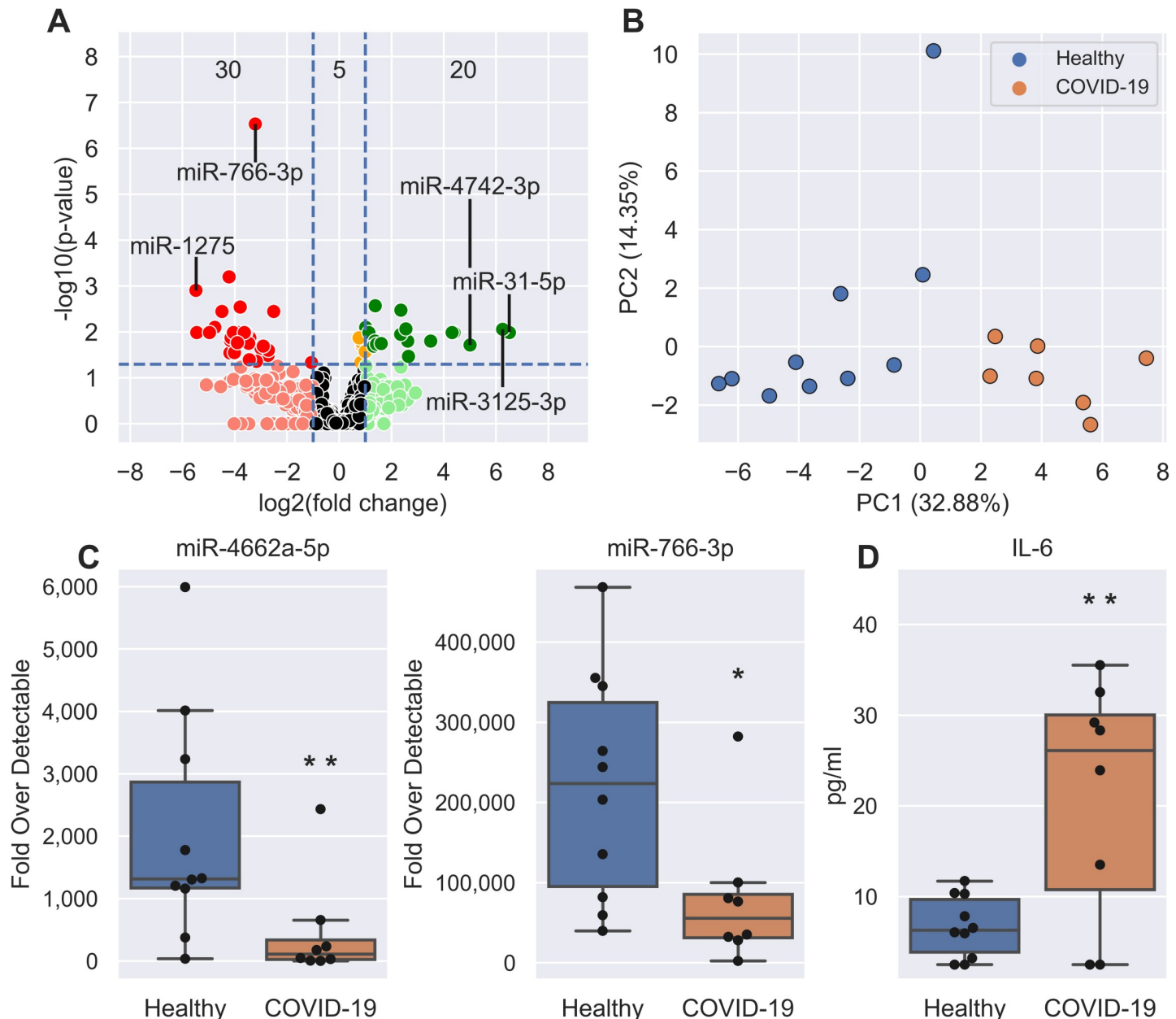
Fig 1. SARS-CoV-2 induces circulating miRNA and cytokine changes. A , Volcano plot showing the increased (green) and decreased (red) DE miRNAs in V1 COVID-19 patients when compared to healthy controls. Horizontal dotted line is the p-value cut-off (False Discovery Rate, FDR < 0.05) and the vertical lines are the fold change cut-off (> 2 FC). Orange miRNAs are statistically significant but are not > 2 FC. The number of statistically significant miRNAs (adjusted P-value < 0.05) in each section are shown: < -1 Log 2 FC (30 miRNAs), between -1 and 1 Log 2 FC (5 miRNAs), and > 1 Log 2 FC (20 miRNAs). The most up-regulated, down-regulated, and statistically significant miRNAs have been labelled. B , PCA plot showing the separation of healthy (blue, n = 10) and COVID-19 V1 (orange, n = 7) samples using the 55 DE miRNAs. C-d , Boxplots of (C) select qRT-PCR validated miRNAs and (D) IL-6 expression in healthy (blue, n = 10) and COVID-19 V1 (orange, n = 8) samples. Boxes are the 25 th - 75 th percentile, line is the median, and whiskers are 1.5x IQR. * p-value < 0.05, ** p-value < 0.01.
