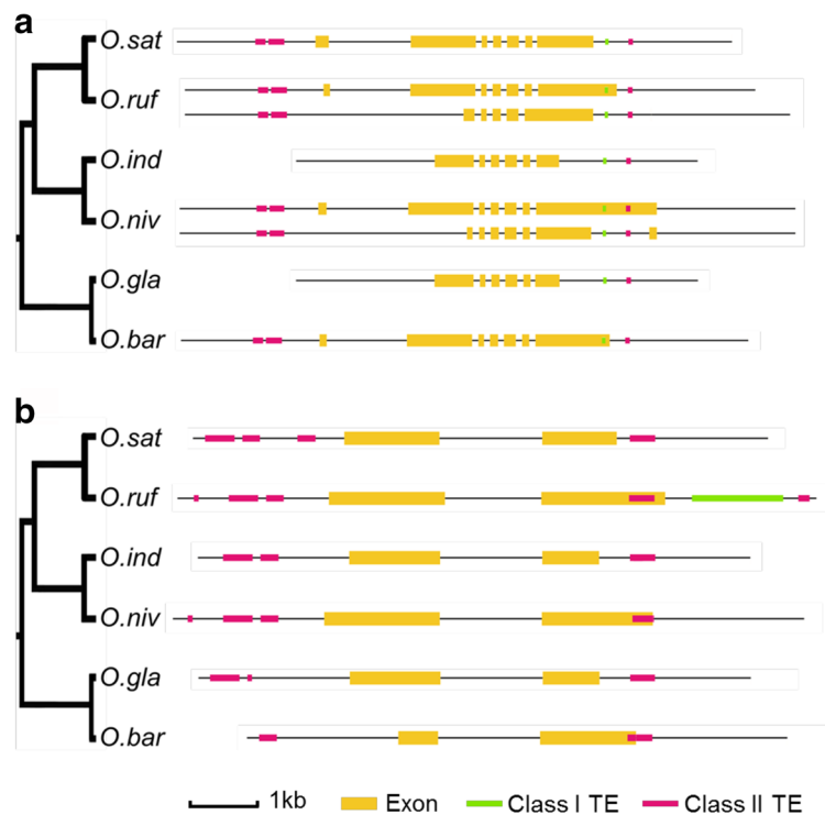
Fig. 5 Pair-wise comparisons of gene structure and TE locations of two examples within GO:0016301. a LOC_Os07g48290 gene. b LOC_Os02g45750 gene
