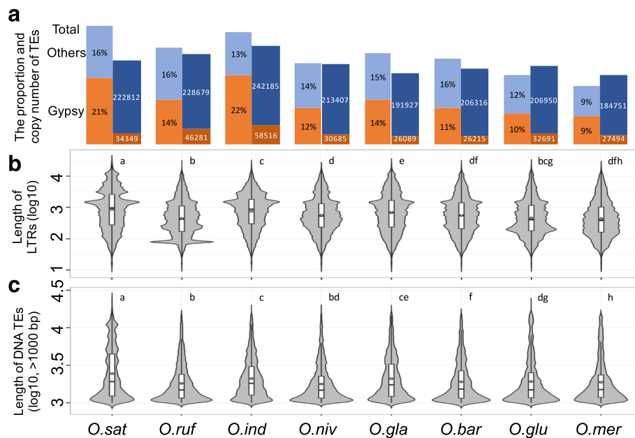
Fig. 2 TEs occupy more space in cultivated rice genomes as compared to their wild relatives. a The proportion and copy number of Gypsy and Total TEs in the different rice genomes. The left bars represent relative amounts of Gypsy and Total TE sizes compared to the genome sizes, and the right bars represent the number of Gypsy and Total transposons in the respective genomes. b-c Violin graphs of the length of LTR transposons ( b ), and DNA transposons ( c ), in the different rice genomes. The violin bars followed by the same letter are not significantly different ( P < 0.05 ) as determined by Student's t test
