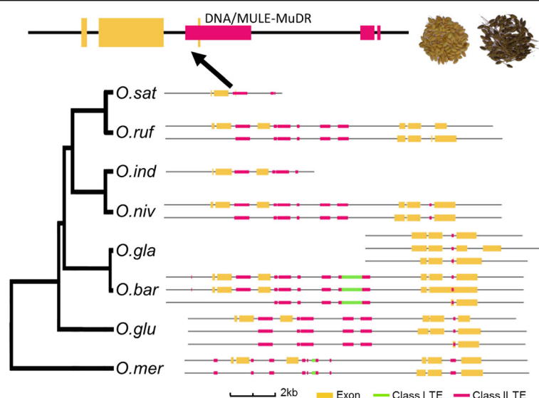
Fig. 7 Comparison of gene structure and TE locations of BH4 gene critical for grain filling in the eight rice species. Organization of exons, introns and TEs of BH4 ( BLACK HULL4 ; LOC_Os04g38660) gene in gene body and 2-kbp flanking sequences of the gene. A blown-up image of BH4 gene structure of O. sativa Japonica is shown above the main image. This mutation changed the black-colored seed hull of the ancestral wild rice to the straw-white seed hull of cultivated rice
