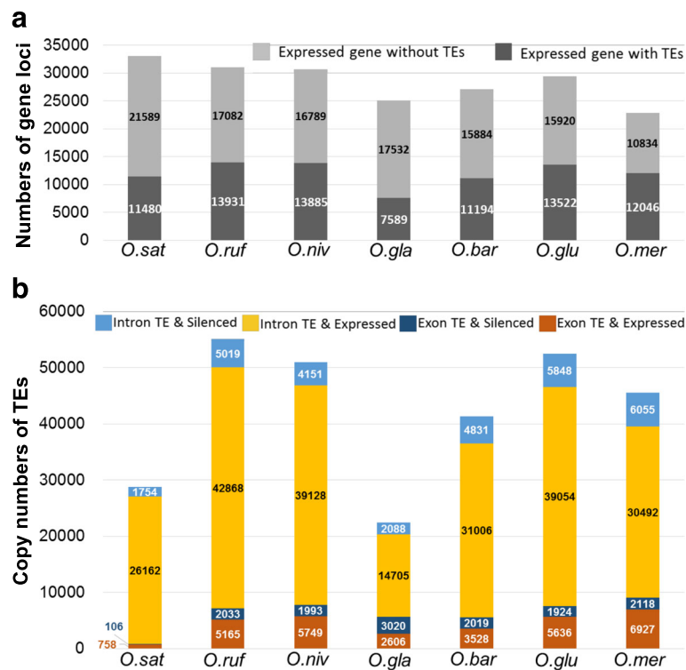
Fig. 4 TEs are preferentially located to intronic gene regions. a Expressed genes with or without TEs. b Numbers of TEs in expressed or not expressed genes based on RNA-seq transcriptomic data
