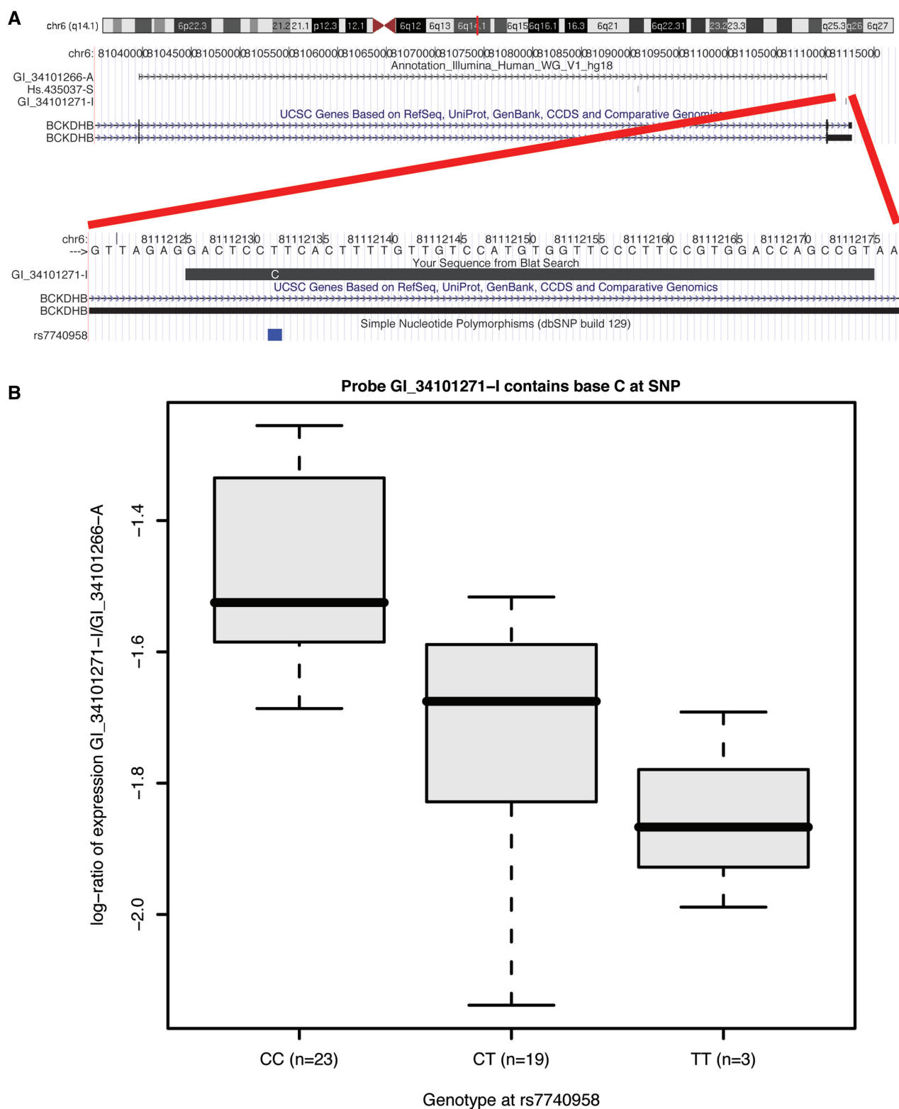
Figure 3. Association between genotype and measured expression. (A) The sequence we examine is in the BCKDHB gene on chromosome 6, which contains a SNP (rs7740958—T/C) at position 7. The Illumina probe targeting this sequence (GI_34101271-I) contains a C at this location. There is also a probe (GI_34101266-A) targeting a constitutive splice junction of BCKDHB and matching no known SNPs. [Figure built based on UCSC Genome Browser graphics (26).] (B) Box plots of the \log_2 expression ratios in the Japanese HapMap population according to the rs7740958 genotype.
