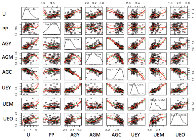
Fig. 6 Scatterplot of Melbourne Data Part II
