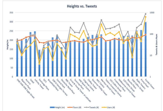
Fig. 7 Correlation between Skyscraper Height and Tweeters
