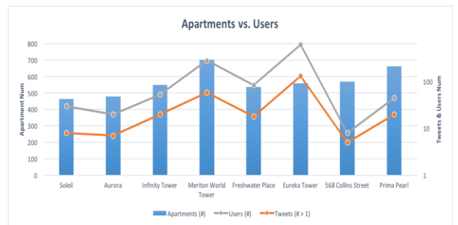
Fig. 8 Correlation between #Skyscraper Apartments and Tweeters
