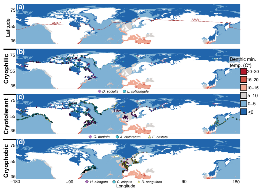
FIGURE 1 (a) Benthic minimum temperature regimes used to define the Arctic environment (<0°C), along with occurrence records used to train models of marine forest distributions under climate change according to affinity to the Arctic environment, including (b) cryophilic, (c) cryotolerant, and (d) cryophobic species. Records are overlaying Bio-ORACLE layer benthic long-term minimum annual temperature (C°; min. depth). Records are derived from Lüning (1990), digitized herbarium records ( https://macroalgae.org/portal/ ; this study), among other databases (see methods). Records were further curated based on DNA barcode insights (Bringloe & Saunders, 2018; Bringloe et al., 2020). The red dashed line defines the Arctic basin, as per AMAP (1998)
