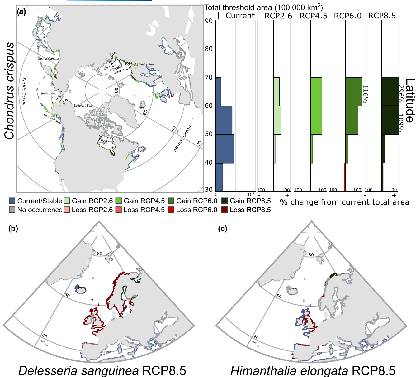
FIGURE 4 Species model projections under various Representative Concentration Pathway (RCP) scenarios by the end of the century (2100) in cryophobous marine forest species, including (a) Chondrus crispus , (b) Delesseria sanguinea , and (c) Himanthalia elongata . Per cent gains and losses in the total threshold area according to latitude are also presented for Chondrus crispus . Present-day predicted threshold occurrence is depicted in blue (stable) or red (loss under climate change). All areas considered (coloured and dark grey) represent the environmental layers analysed, masked for depth (>100 m) or distance from shore (>10 km), and depositional substrate (sand/mud) as per Nyberg and Howell (2016). For individual species responses according to RCP scenarios, please refer to results provided on FigShare ( https://doi.org/10.6084/m9.figshare.14751753.v6 )
