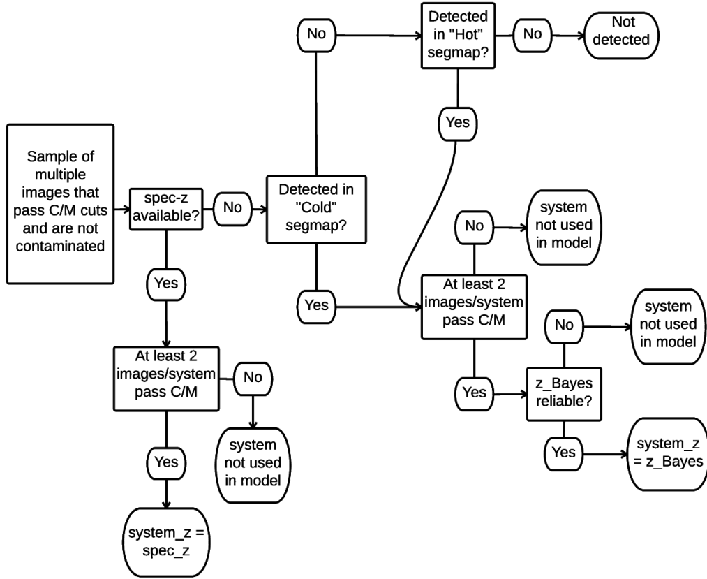
FIG. 4.—: Flow chart describing our procedure for assigning photometric redshifts to multiple image systems. Two segmentation maps, a “hot” and a “cold” version, were used for source detection. The detection and deblending thresholds are set to the SExtractor defaults in the cold segmentation map. Objects detected in the cold segmentation map, typically the brighter and more isolated ones, have more accurate photometry. The hot segmentation map was created using extremely aggressive detection and deblending thresholds. It detects the majority of the remaining multiple images that are not detected in the cold version. C/M cuts refer to the color/morphology cuts used to purify the sample of multiple images. z_{\text{Bayes}} refers to the redshift obtained from combining multiple redshifts in a hierarchical Bayesian model (Dahlen et al. 2013). z_{\text{Bayes}} is considered reliable if it is larger than the redshift of Abell 2744, z = 0.308 , and it is not multi-valued. See the Appendix for examples of multiple image systems that pass and fail some of the tests in this flow chart.
