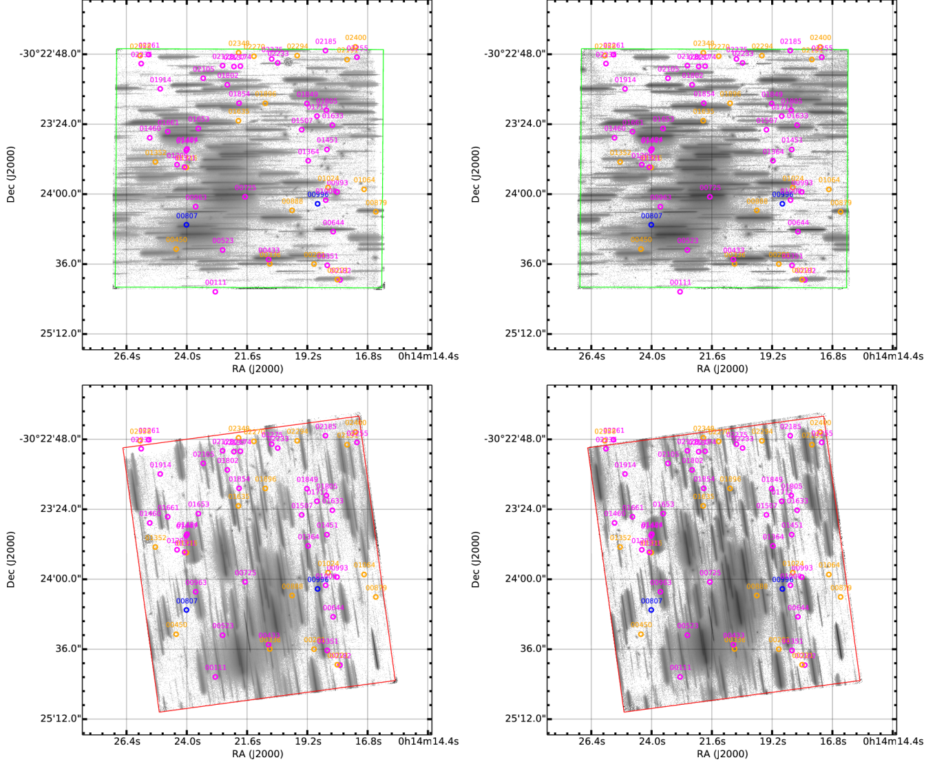
FIG. 2.—: The GLASS G102 (left) and G141 (right) grism pointings of Abell 2744 at two distinct P.A.s, with field-of-view shown by the red (P.A.=233 degrees) and green (P.A.=135 degrees) squares. The circles in all panels denote the positions of the emission line objects identified in this work, with color coding following the convention adopted in Figure 1.
