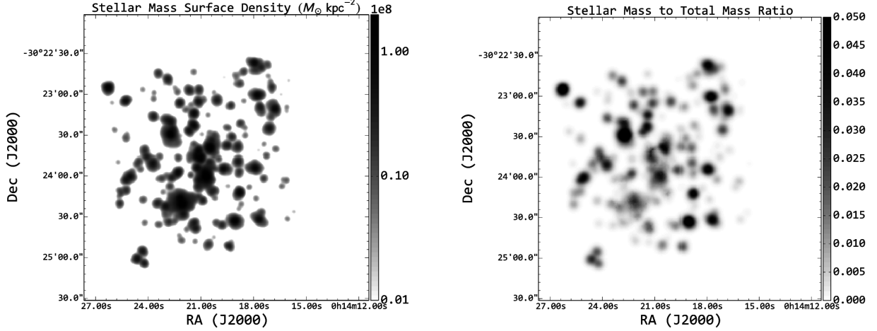
FIG. 15.—: Stellar mass surface density (left) and stellar to total mass ratio (right) distributions of Abell 2744. Stellar mass surface density is in the unit of M_{\odot} \text{ kpc}^{-2} .
