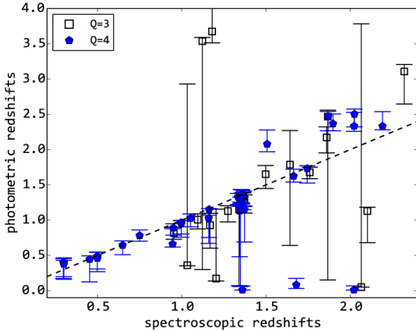
FIG. 10.—: Comparison between the spectroscopic and photometric redshifts for the 55 objects with high-confidence emission lines (quality flags 3 or 4). We also show the 1\text{-}\sigma error bars (enclosing 68% of the total probability) around the photometric redshifts. There is reasonably good agreement between photometric and spectroscopic redshifts, with 25 out of 55 spectroscopic redshifts within the photometric redshift error bars. This is acceptable considering that the photometric redshift uncertainties only include the random component, even though they suggest that an additional systematic uncertainty component is present. In order to account for this systematic uncertainty, for the systems used to build the lens model we added 20% in quadrature to our photometric errors.
