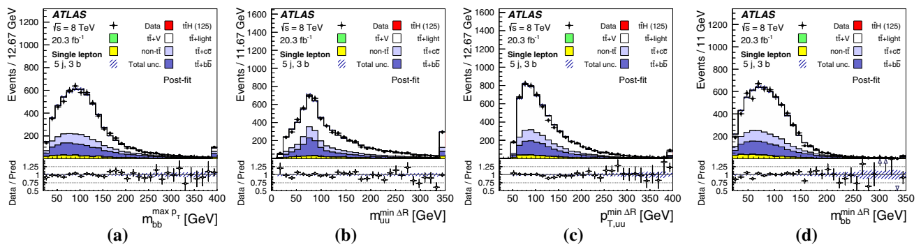
Fig. 28 Single-lepton channel: post-fit comparison of data and prediction for the four top-ranked input variables in the (5j, 3b) region. The plots include a m_{bb}^{\max p_T} , b m_{uu}^{\min \Delta R} , c p_{T,uu}^{\min \Delta R} and d m_{bb}^{\min \Delta R} . The first and last bins in all figures contain the underflow and overflow,
