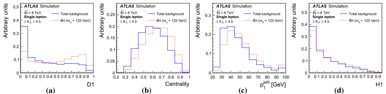
Fig. 24 Single-lepton channel: comparison of t\bar{t}H signal ( dashed ) and background ( solid ) for the four top-ranked input variables in the (\geq 6j, \geq 4b) region. The plots include a D1 , b Centrality, c p_T^{\text{jet}5} , and d H1
