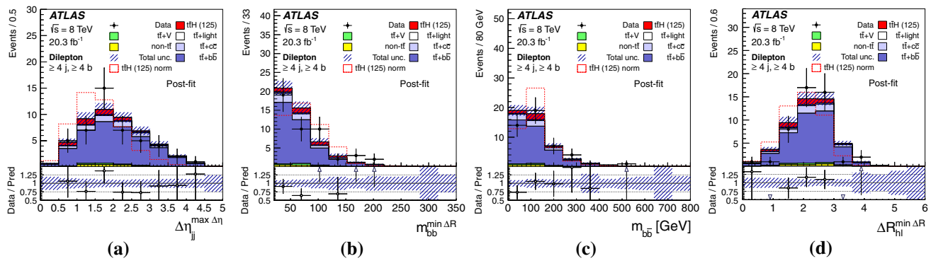
Fig. 34 Dilepton channel: post-fit comparison of data and prediction for the four top-ranked input variables in the ( \geq 4j, \geq 4b ) region. The plots include a \Delta\eta_{jj}^{\max} \Delta\eta , b m_{bb}^{\min} \Delta R , c m_{bb} , and d \Delta R_{hl}^{\min} \Delta R . The first and last bins in all figures contain the underflow and overflow, respectively. The bottom panel displays the ratio of
