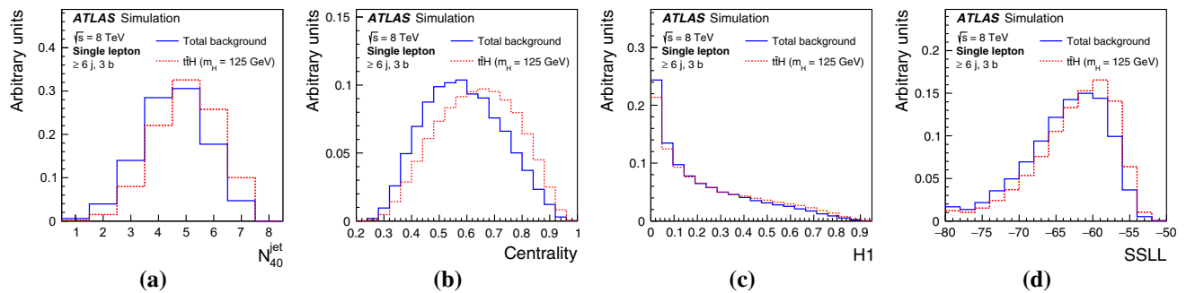
Fig. 23 Single-lepton channel: comparison of t\bar{t}H signal ( dashed ) and background ( solid ) for the four top-ranked input variables in the (\geq 6j, 3b) region. The plots include a N_{40}^{\text{jet}} , b Centrality, c H1 , and d SSLL
