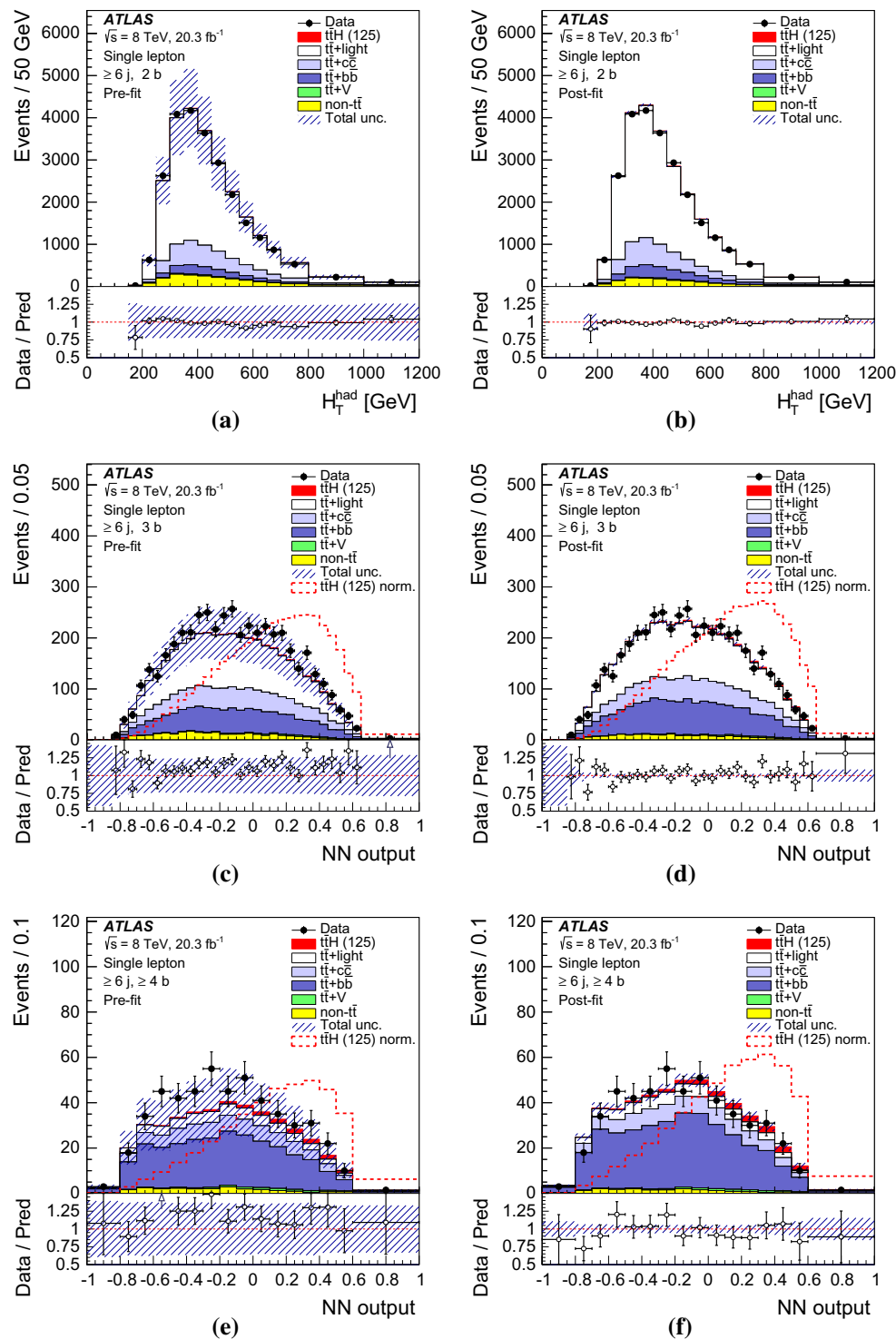
Fig. 13 Single-lepton channel: comparison of data and prediction for the discriminant variable used in the ( \geq 6j , 2b) region a before the fit and b after the fit, in the ( \geq 6j , 3b) region c before the fit and d after the fit, in the ( \geq 6j , \geq 4b ) region e before the fit and f after the fit. The fit is performed on data under the signal-plus-background hypothesis. The last bin in all figures contains the overflow. The bottom panel displays the ratio of data to the total prediction. An arrow indicates that
