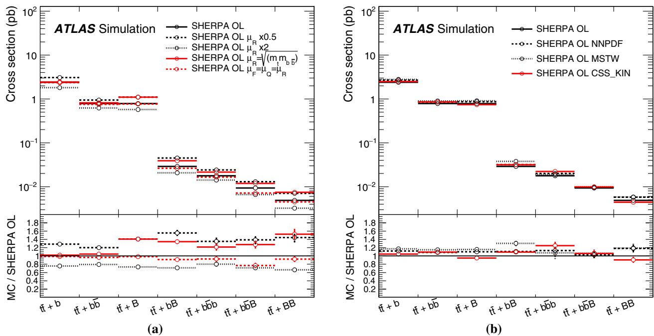
Fig. 9 Systematic uncertainties on the t\bar{t} + b\bar{b} contribution based on a scale variations and b PDF choice and shower recoil model of the SHERPAOL simulation. The effect of a given systematic uncertainty is shown
