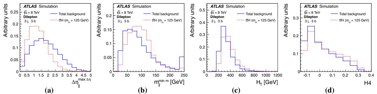
Fig. 25 Dilepton channel: comparison of t\bar{t}H signal ( dashed ) and background ( solid ) for the four top-ranked input variables in the (3j, 3b) region. The plots include a \Delta\eta_{jj}^{\text{max} \Delta\eta} , b m_{jj}^{\text{min} m} , c H_T , and d H4
