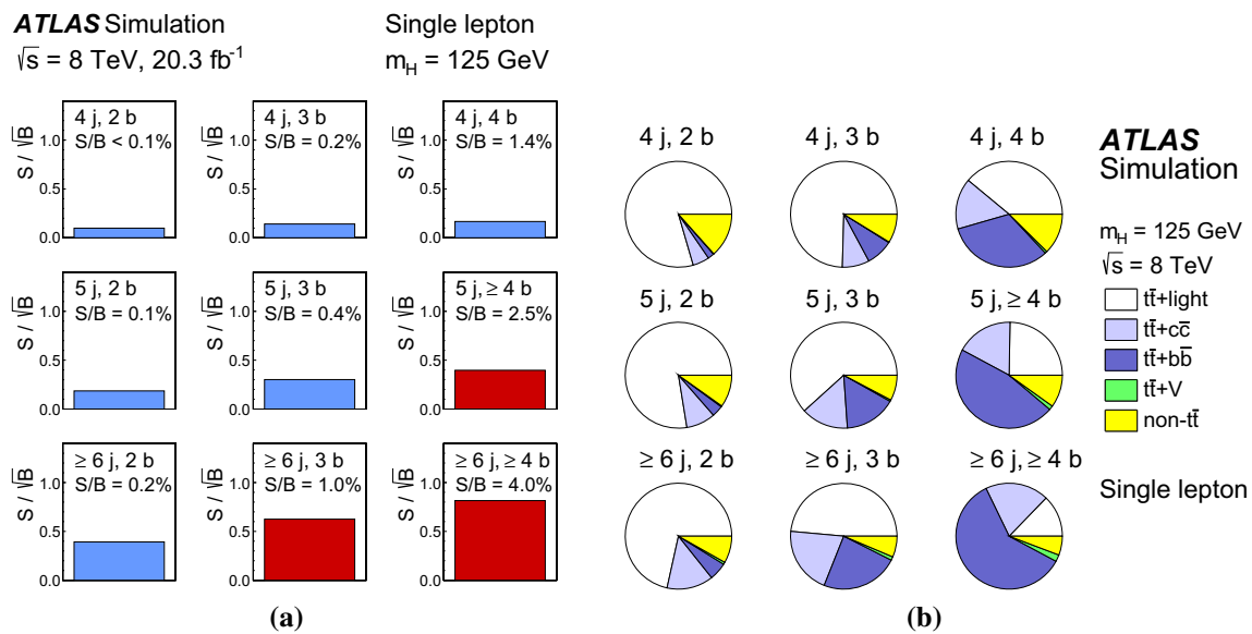
Fig. 2 Single-lepton channel: a S/\sqrt{B} ratio for each of the regions assuming SM cross sections and branching fractions, and m_H = 125 GeV. Each row shows the plots for a specific jet multiplicity (4, 5, \geq 6 ), and the columns show the b -jet multiplicity (2, 3, \geq 4 ). Signal-rich regions are shaded in dark red, while the rest are shown in light blue.
