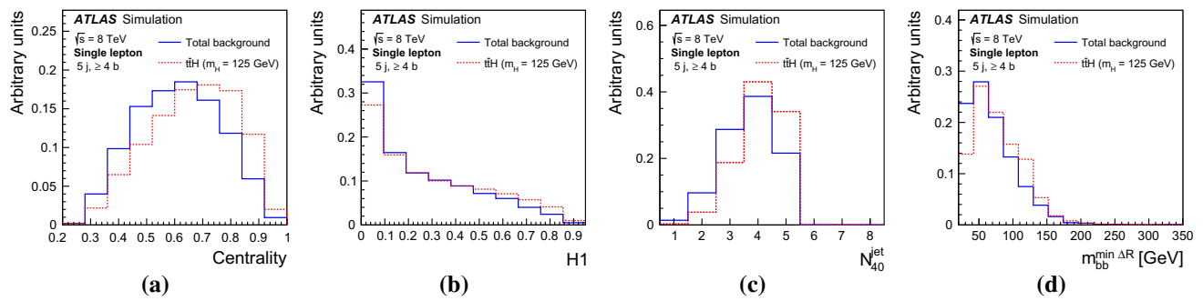
Fig. 22 Single-lepton channel: comparison of t\bar{t}H signal ( dashed ) and background ( solid ) for the four top-ranked input variables in the (5j, \geq 4b) region. The plots include a Centrality, b H1 , c N_{40}^{\text{jet}} and d m_{bb}^{\text{min} \Delta R}
