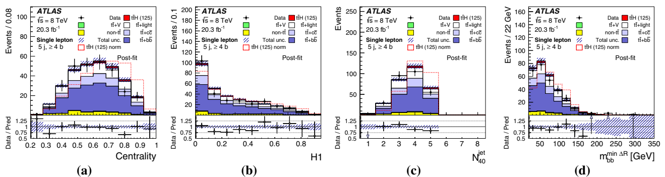
Fig. 29 Single-lepton channel: post-fit comparison of data and prediction for the four top-ranked input variables in the (5j, \geq 4b ) region. The plots include a Centrality, b H1 , c N_{40}^{\text{jet}} and d m_{bb}^{\min \Delta R} . The first and last bins in all figures contain the underflow and overflow, respectively. The bottom panel displays the ratio of data to
