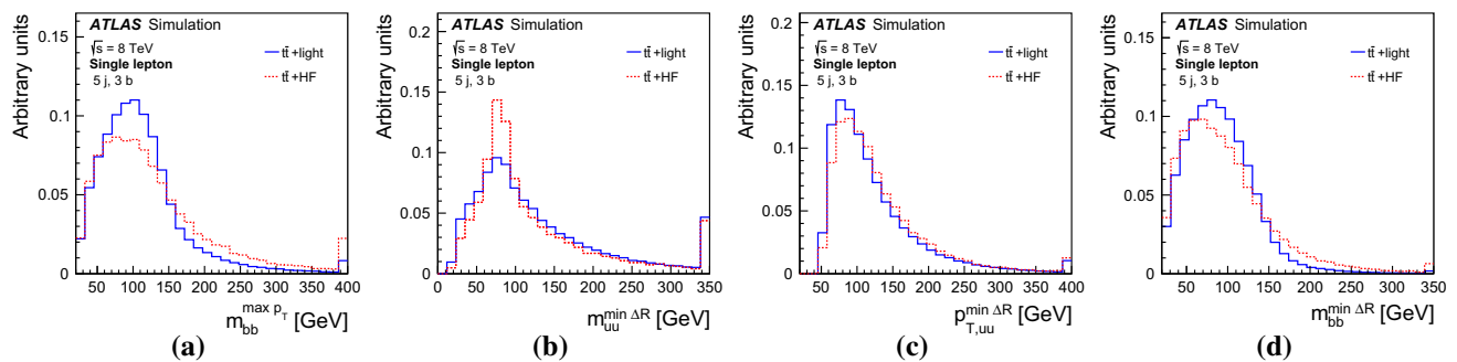
Fig. 21 Single-lepton channel: comparison of t\bar{t} + \text{HF} (dashed) and t\bar{t} + \text{light} (solid) background for the four top-ranked input variables in the (5j, 3b) region where the NN is designed to separate these two backgrounds. The plots include a m_{bb}^{\max p_T} , b m_{uu}^{\min \Delta R} , c p_{T,uu}^{\min \Delta R} and d m_{bb}^{\min \Delta R}
