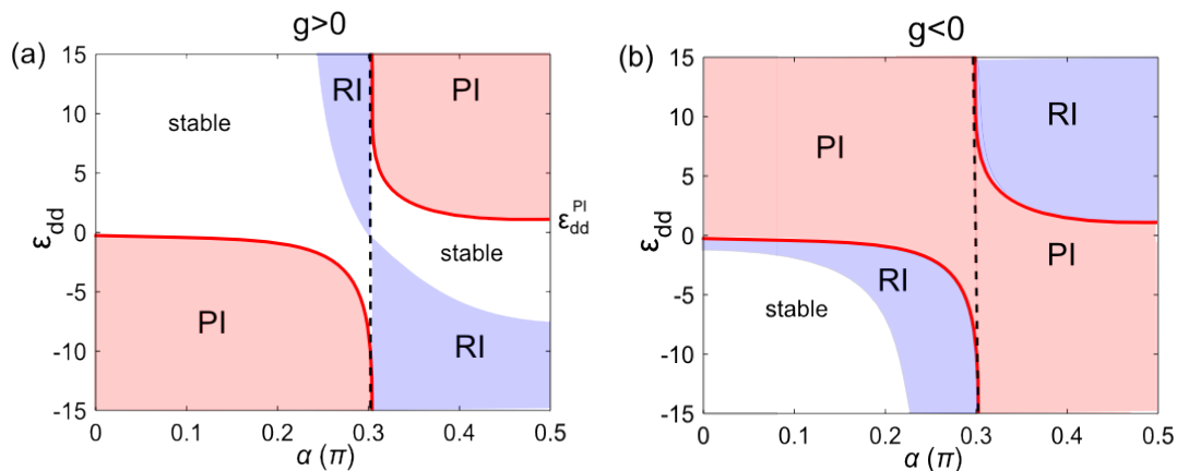
Figure 2. Stability diagram in \varepsilon_{dd} - \alpha space for the homogeneous 2D dipolar BEC ( \sigma = 0.5 ) with (a) g > 0 and (b) g < 0 . Shown are the regions of stability (white), phonon instability (pink) and roton instability (blue). The threshold for the phonon instability \varepsilon_{dd}^{PI} = [1 - 3 \cos^2 \alpha]^{-1} is shown by the red lines. The vertical dashed line indicates the magic angle \alpha_0 . Note that the plots only extend up to \alpha = \pi/2 ; beyond this the results are the mirror image of the presented region.
