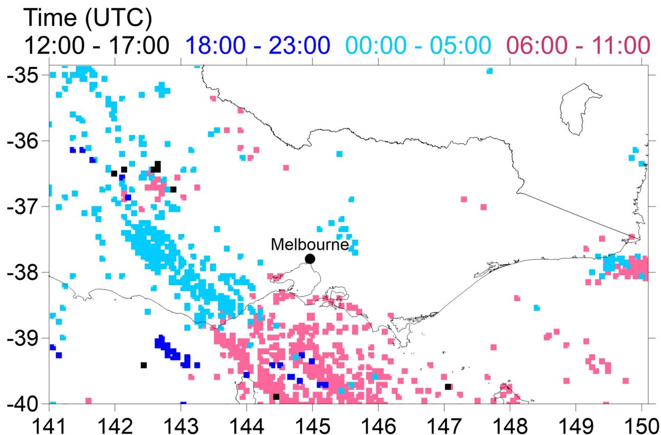
Fig 7. Location of lightning occurrences in 6-hourly blocks starting late 20 November into 21 November 2016. The pink pixels coincide with timing of the storm passing Melbourne. Basemap from Igismap.com 2020.
