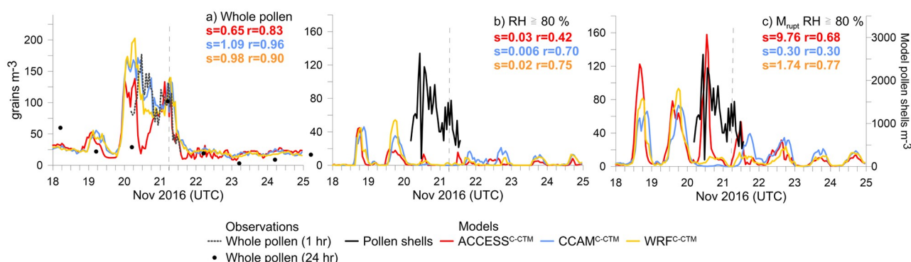
Fig 2. Time series in whole grass pollen (a) and pollen shells (b–c) from the RH \geq 80\% experiment. Panel (b) shows results from in-atmosphere only pollen rupturing, whilst panel (c) includes the on-plant mechanical rupturing from Eqs 2–5. Model values in (c) are on second y-axes to the right. s = slope of the linear regression and r = r correlations between modelled and observed pollen (or pollen shells), given in same colours as the legend. Vertical dashed line indicates the time of the storm.
