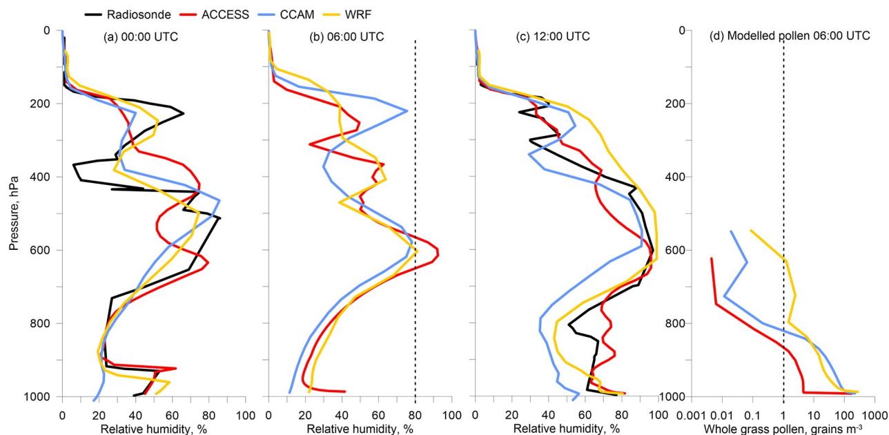
Fig 4. (a-c) radiosonde observations at Melbourne Airport compared to model predictions for the 21 November 2016 of relative humidity from the surface to 0 hPa in each meteorological model. (d) pollen concentrations in VGPEM1.0 driven by each meteorological model. Dashed lines in (b) and (d) represent the thresholds for rupturing at 80% RH and 1 grain m -3 , respectively. The maximum height of modelled pollen differs because CCAM and WRF are output on pressure levels, whilst the ACCESS height is converted to hPa from the 5 km model level.
