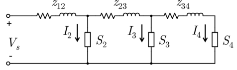
Fig. 2. Simple network.
