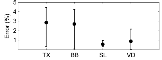
Fig. 10. Constraint errors due to linearization, for transformer capacity (TX), backbone current rating (BB), service line rating (SL), and voltage drop (VD).
