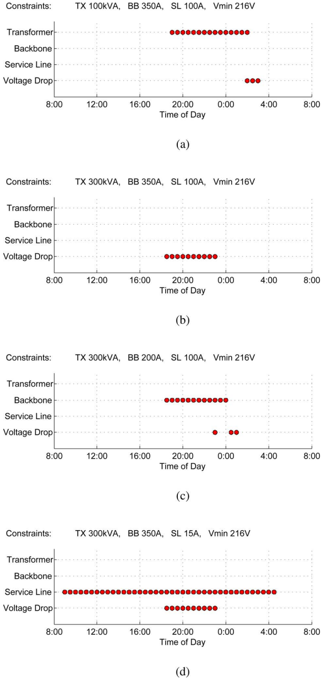
Fig. 9. Active constraints for four separate scenarios. (a) Active constraints for a scenario in which transformer capacity is the main limitation. (b) Active constraints for a scenario in which voltage drop is the main limitation. (c) Active constraints for a scenario in which the backbone's current rating is the main limitation. (d) Active constraints for a scenario in which the service line's current rating is the main limitation.
