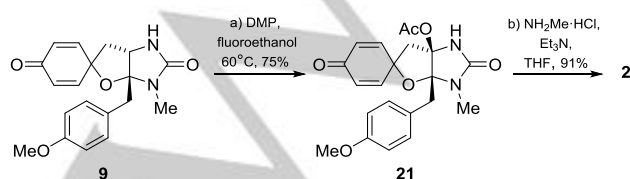
Scheme 4. DMP mediated cyclic urea oxidation and completion of the total synthesis.
