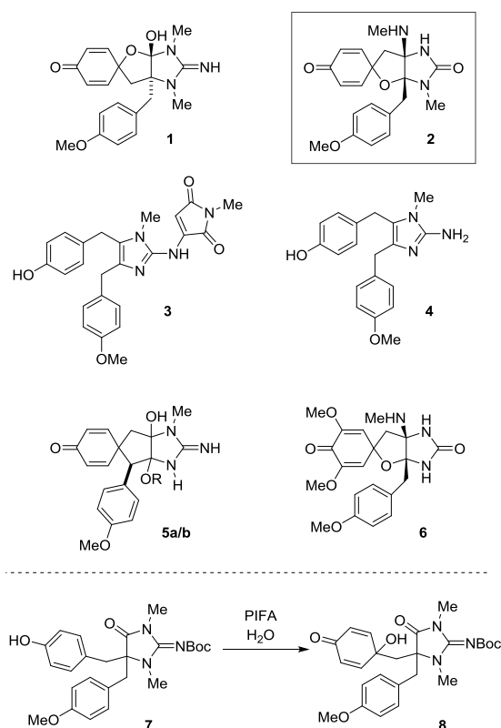
Figure 1. Originally assigned structure (1) and revised structure (2) of spiroleucettadine, representative Leucetta alkaloids naamidine A (3), naamine A (4), spirocalcardine A (5a, R = OMe), spirocalcardine B (5b, R = OH), spironaamidine (6) and failed oxidative spirocyclization towards 1.
