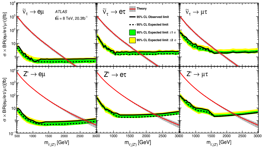
FIG. 2 (color online). The 95% C.L. limits on cross section times branching ratio as a function of \tilde{\nu}_\tau mass (top plots) and Z' mass (bottom plots) for e\mu (left), e\tau (middle), and \mu\tau (right). Theory curves are for the arbitrary choice of couplings \lambda'_{311} = 0.11 and \lambda_{i3k} = 0.07 for \tilde{\nu}_\tau and Q_{\ell\ell'} = 1 for Z' . The gray band around the theory curve represents the theoretical uncertainty from the PDFs and factorization and renormalization scales.
