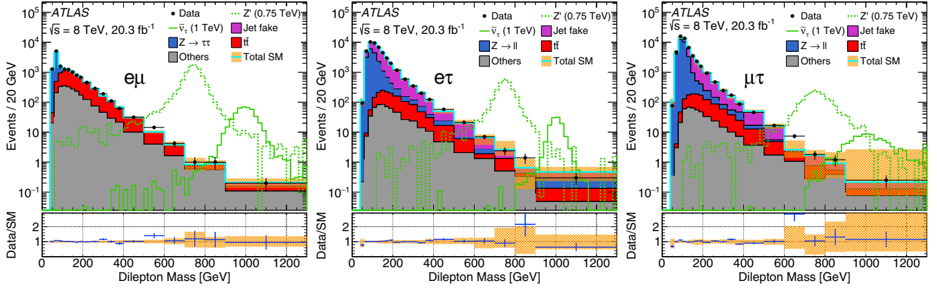
FIG. 1 (color online). Observed and predicted e\mu , e\tau , \mu\tau invariant mass distributions. The contributions of the different processes are also shown: “Others” includes diboson and single-top while “Jet fake” refers to W + jets and multijet. All overflows are included in the rightmost bin. Signal simulations are shown for m_{\tilde{\nu}_\tau} = 1 TeV and m_{Z'} = 0.75 TeV. The couplings \lambda'_{311} = 0.11 and \lambda_{i3k} = 0.07 ( Q_{\ell\ell'} = 1 ) are used for the RPV ( Z' ) model. The uncertainty bands include both the statistical and systematic uncertainties.
