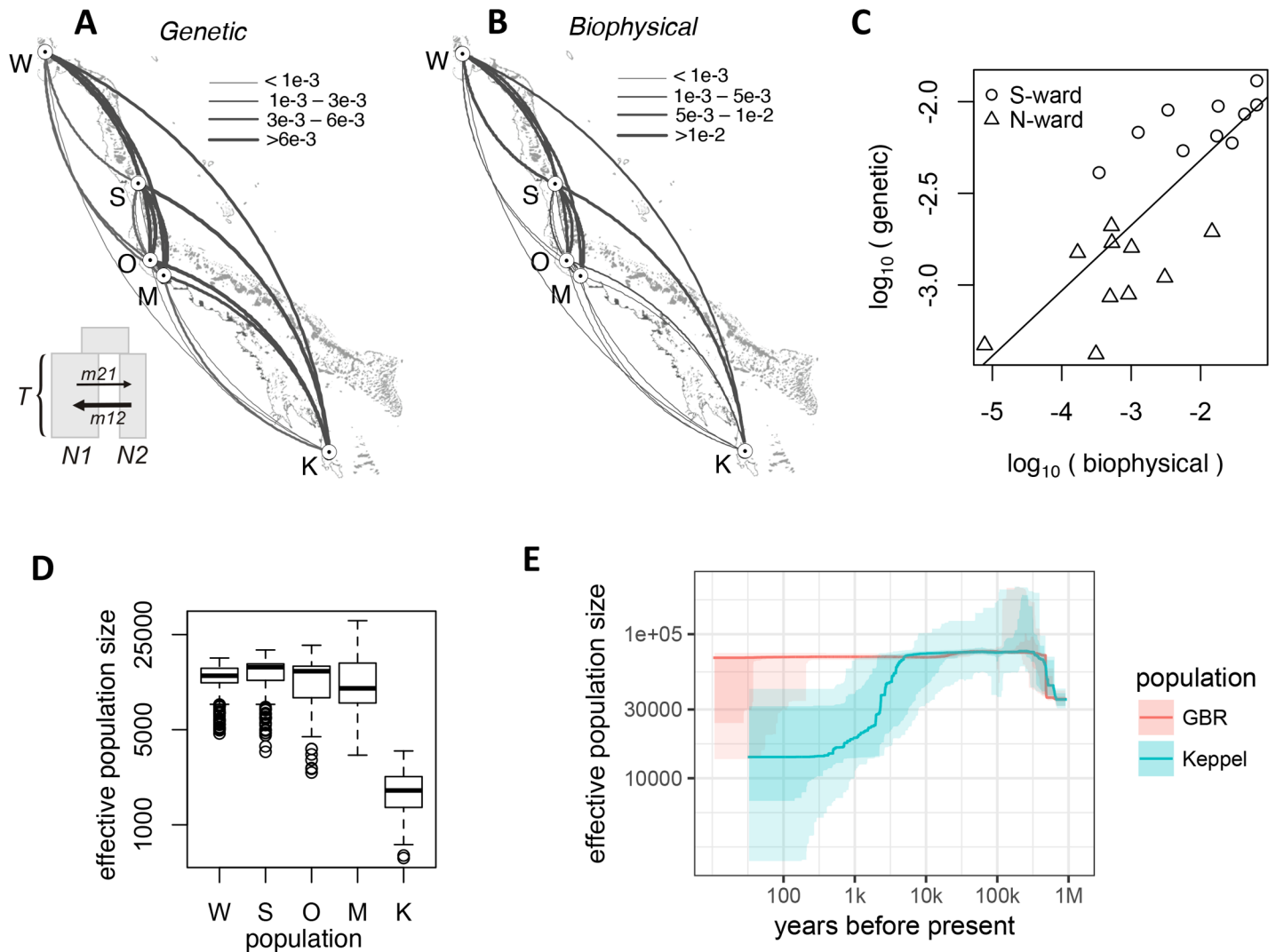
Fig 2. Estimated demography of A. millepora populations on the GBR. (A) Arc-plot of migration rates among populations reconstructed from population genomic data. Inset: \partial\text{adi} model used: ancestral population splits into two populations of unequal sizes (N1 and N2) some time T in the past, these populations exchange migrants at different rates depending on direction. (B) Migration rates according to the biophysical model. On panels A and B, the arcs should be read clockwise to tell the direction of migration; line thickness is proportional to the migration rate. (C) Correlation between log-transformed biophysical and genetic migration rates (Mantel r = 0.58 , P = 0.05 ). (D) Box plot of effective population sizes inferred by the split-with-migration model (panel A) across all population pairs and bootstrap replicates. (E) Historical effective population sizes inferred by stairwayPlot for the Keppel population and pooled Sudbury, Orpheus and Magnetic populations (GBR). The line is median of 200 bootstrap replicates, light shaded area is 95% credible interval, dark-shaded area is 75% credible interval.
