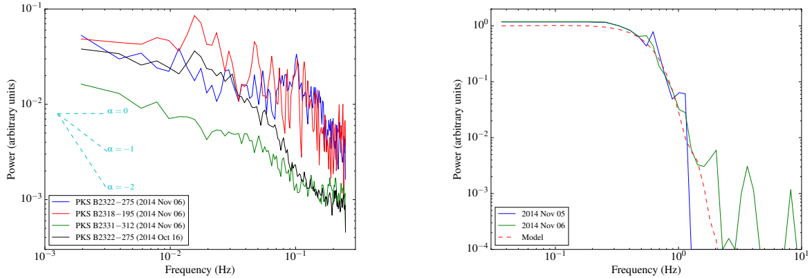
FIG. 3.— Left: temporal power spectra of the flux densities for PKS B2322–275 (blue, with 62 min of data), PKS B2318–195 (red, with 37 min of data), and PKS B2331–312 (green, with 235 min of data), using the data from Figure 2 when large-amplitude scintillations are evident. The power spectra are estimated using Welch’s method, averaging spectra with 256 data-points and 50% overlap. We also show the power spectrum of PKS B2322–275 from our comparison night (black). The cyan dashed lines show power-laws with slopes \alpha = 0 , -1 , and -2 as labeled. Right: temporal power spectra of the flux density for PKS B2211–388, measured by the Ooty radio telescope at 327-MHz. The power spectrum for 2014 November 05 (blue) shows substantially less power above 1 Hz than that for 2014 November 06 (green); note that both power spectra have been normalized below 0.1 Hz). The model fit (red dashed line) is for a solar wind velocity of \approx 500 \text{ km s}^{-1} .
