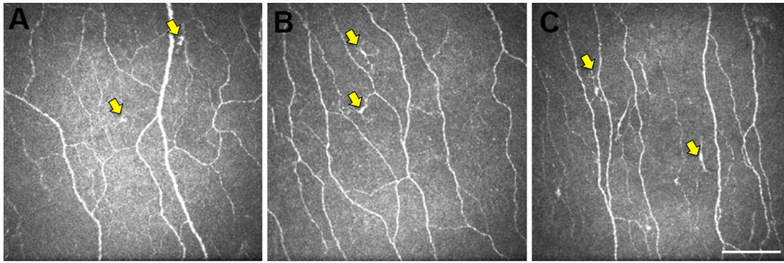
FIGURE 2 | Representative central corneal IVCN images. Images of the central corneal sub-basal nerve plexus from participants in the CN (A), MCI (B), and AD (C) groups. The epithelial DCs (yellow arrows) are smaller and less stratified in CN eyes (A) relative to the larger more stratified morphology of DCs in MCI and AD eyes. Scale bar: 100 \mu\text{m} , applies to all images.
