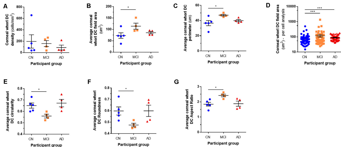
FIGURE 3 | Corneal whorl dendritic cell parameters. Corneal DC density in the mid-peripheral inferior whorl region (A) was similar amongst the cognitive normal (CN), mild cognitive impairment (MCI), and Alzheimer's disease (AD) participant groups. On average, the corneal DCs had a larger field area (B) and perimeter (C) in MCI eyes, relative to CNs. In the "per cell" analysis, DCs from CNs had smaller field areas than cells from individuals with MCI and AD (D). In addition, DCs in the inferior whorl region of MCI eyes were less circular (E), less round (F), and had a higher aspect ratio (G) than DCs in CNs. p < 0.05 , ***p < 0.001 .
