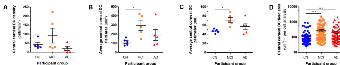
FIGURE 1 | Central corneal dendritic cell parameters. Central corneal DC density ( A ) was similar amongst the cognitive normal (CN), mild cognitive impairment (MCI), and Alzheimer's disease (AD) participants groups. On average, central corneal DCs had a larger field area ( B ) and perimeter ( C ) in MCI eyes, relative to CNs. In the “per cell” analysis, central corneal DCs from CNs had significantly smaller field areas than cells from individuals with MCI and AD ( D ). * p < 0.05 , *** p < 0.001 .
