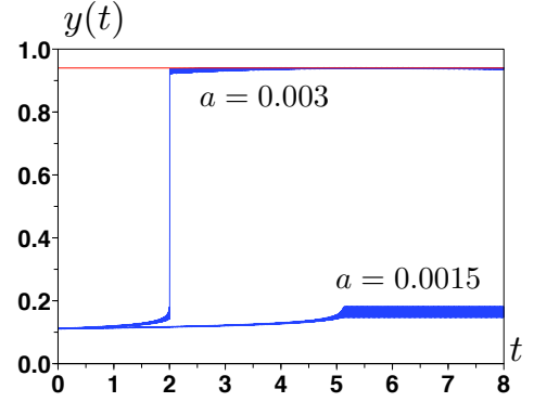
Fig. 17. Output signal y(t) : when a is too small, the trajectory is stuck on the lower branch.
