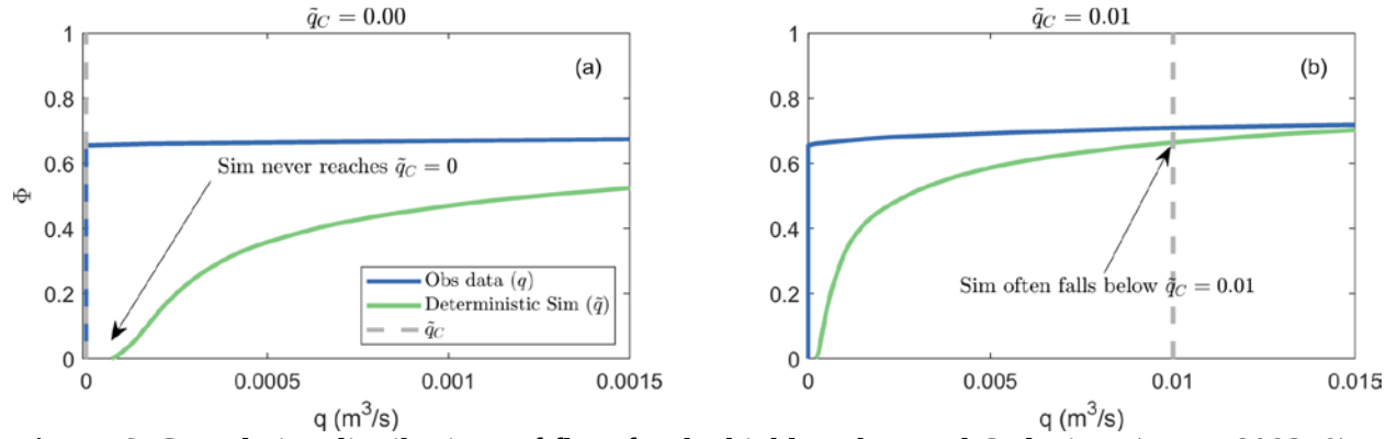
Figure 6. Cumulative distributions of flow for the highly ephemeral Ord River (gauge 809310). Observations (blue line) and deterministic simulations (green line) for the os-censored experiment are shown. Horizontal axes are truncated to focus on very low flow. More than 60% of observations are zero, but when \tilde{q}_C = 0 (left panel), simulations never fall to \tilde{q}_C . The right-hand panel shows that simulations often fall to/below \tilde{q}_C when \tilde{q}_C = 0.01 .
