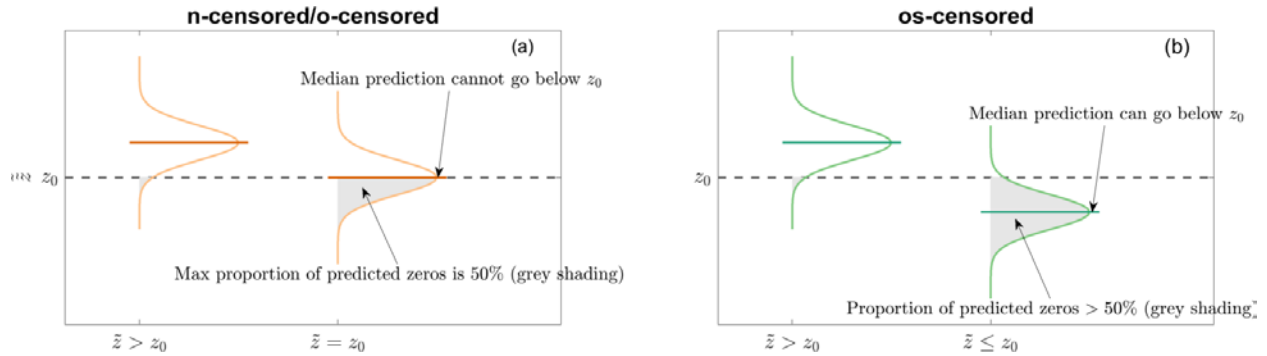
Figure 1. Schematic showing predictive uncertainty under the n-censored/o-censored experiments (panel a) and the os-censored experiment (panel b), where \tilde{z} = M(\tilde{z}) is the median of the Gaussian predictive distribution and z_0 = z_C = \tilde{z}_C = tf[0] . Each panel shows the treatment of predictive uncertainty when \tilde{z} > z_0 and when \tilde{z} \leq z_0 . Only the os-censored case (panel b) allows > 50\% zeros to be generated (see text for explanation).
