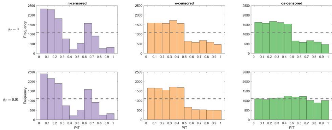
Figure 5. Probability integral transform (PIT) histograms for the highly ephemeral Ord River (gauge 809310). Columns show censoring experiments. Top row shows predictions generated with \tilde{q}_C = 0 , bottom row shows simulations generated with \tilde{q}_C = 0.01 . When PIT values are uniformly distributed (histograms lie along the dashed line), predictions are reliable. Predictions are reliable for the os-censored experiment with \tilde{q}_C = 0.01 (bottom right panel).
