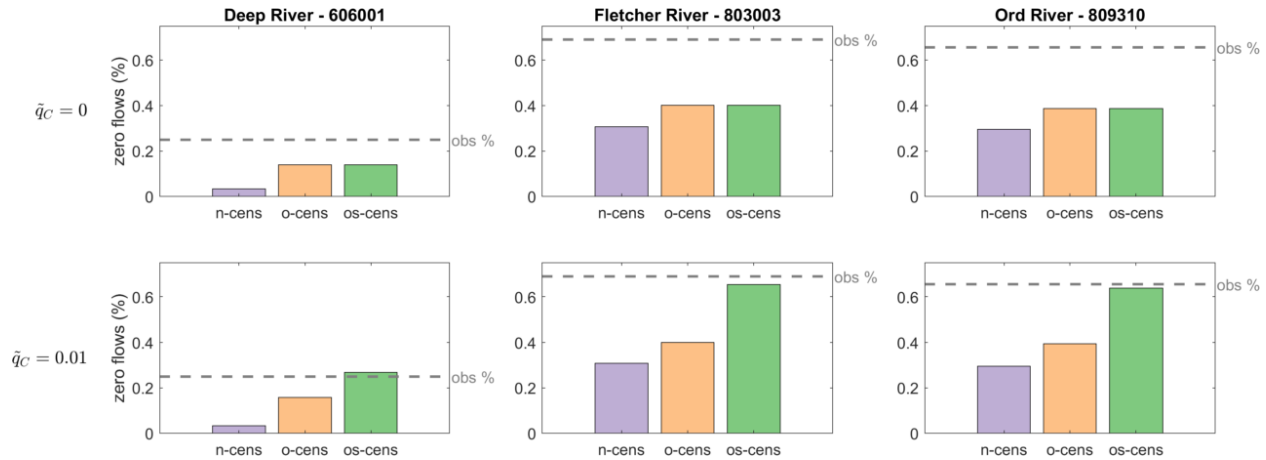
Figure 7. Proportion of zero flow for all gauges (columns). Top row shows predictions generated with \tilde{q}_c = 0 , bottom row shows predictions generated with \tilde{q}_c = 0.01 . Colors show different censoring experiments, and dashed line shows the proportion of zeros in the observed record. The os-censored case with \tilde{q}_c = 0.01 most closely reproduces the proportion of zeros in all catchments.
