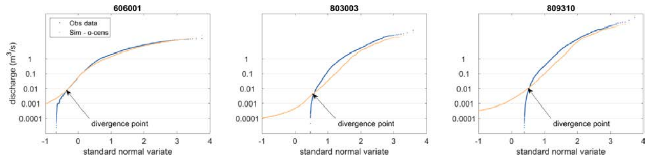
Figure 3. Cumulative frequency distributions of observations and simulations where parameters are estimated with o-censoring. Annotations show the points below which observed and simulated frequency distributions diverge.
