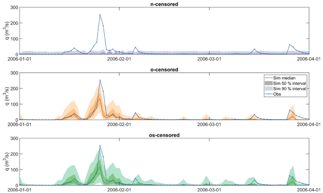
Figure 10. Example simulations for the highly ephemeral Ord River gauge (809310), generated with censoring threshold \tilde{q}_c = 0.01 . Top panel shows n-censored model, middle panel show o-censored model, bottom panel shows os-censored model. The os-censored model produces the most reliable predictions.
