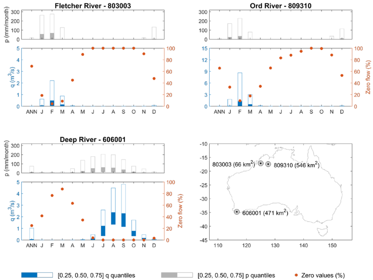
Figure 2. Annual (ANN) and monthly distribution of rainfall (p) and flow (q), including the incidence of zero flow (right-hand axis). Statistics are calculated for the data periods listed for each catchment in Table 1. Catchment locations are given in the bottom right panel.
