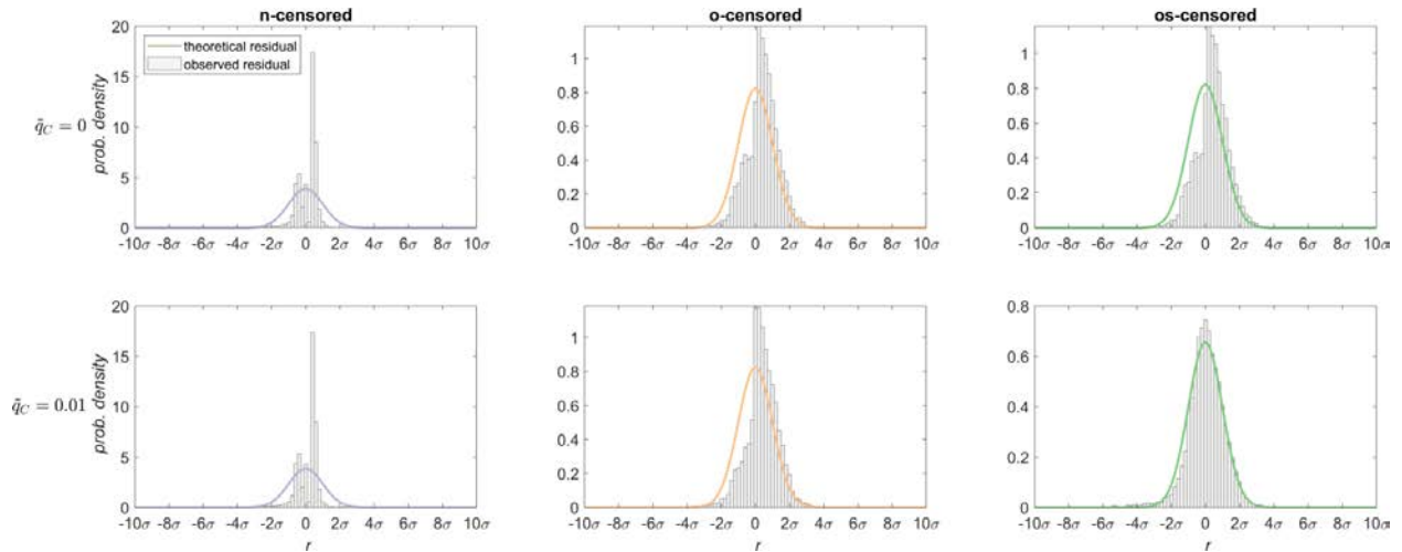
Figure 4. Theoretical and observed residual distributions in the transformed domain for the highly ephemeral Ord River (gauge 809310). Top row shows residuals generated with \tilde{q}_C = 0 ,
