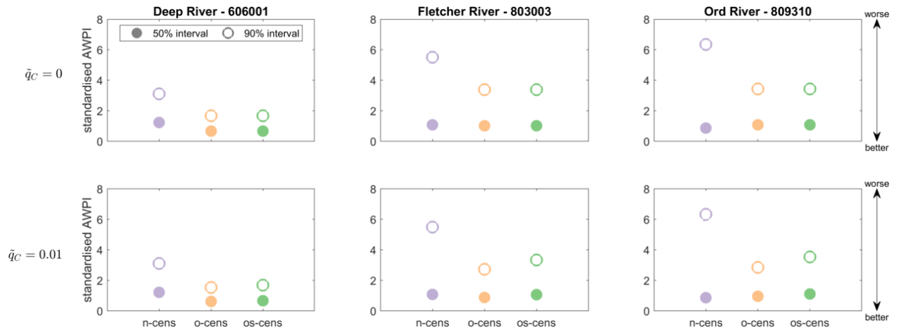
Figure 9. Average width of prediction intervals (AWPI) for 50% (closed circle) and 90% (open circle) intervals, for all gauges (columns). Top row shows predictions generated with \tilde{q}_c = 0 ,
