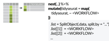
Fig. 2. A cheat sheet of the tidyverse functionalities that tidyseurat enables for Seurat objects. This cheat sheet provides examples of the alternative tidyverse and Seurat syntax. The green colour scheme includes procedures that output a tidyseurat, if: (i) do not lead cell duplication; and (ii) key columns (e.g. cell identifier) are not excluded, modified, nor renamed (e.g. through a select, mutate and rename commands). In this case, a table (rather than an abstraction) is returned for independent analysis and visualization. The blue colour scheme includes procedures that return tibble tables for independent analyses and plotting. The grey-shaded boxes include the alternative code utilizing Seurat and base-R.
