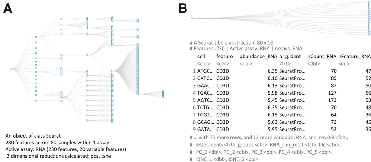
Fig. 1. Comparison between the data structure ( https://github.com/boxuancui/DataExplorer ) (top; abstracted tibble for tidyseurat) and the information presented to the user (bottom) for Seurat (A) and tidyseurat (B; including transcript information). The dataset underlying these visualizations is a subset of a peripheral blood mononuclear cell fraction provided by 10x (10xgenomics.com)
