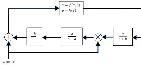
Fig. 3 Basic extremum seeking scheme exhibiting sinusoidal perturbation to plant input, with high and low pass filters either side of demodulation step.
