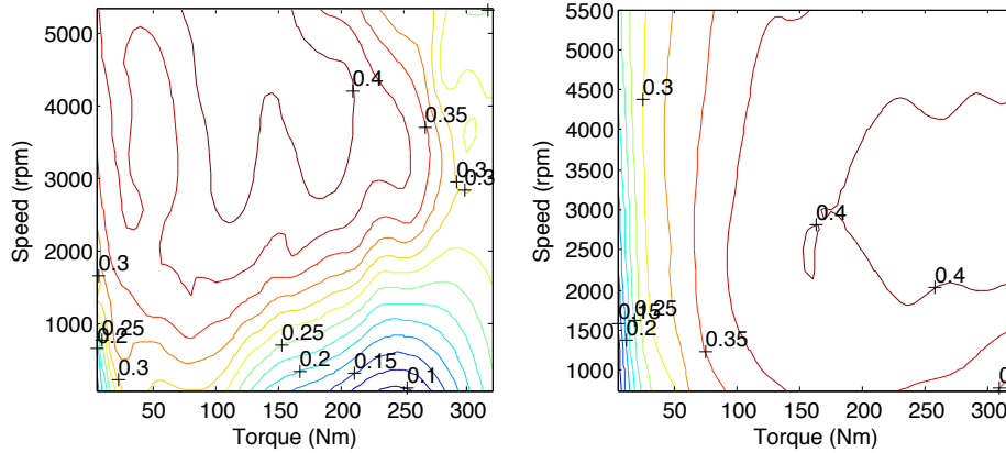
Fig. 2 Engine efficiency maps for a flex fuel engine running with (left) E05 and (right) E85 fuel.
