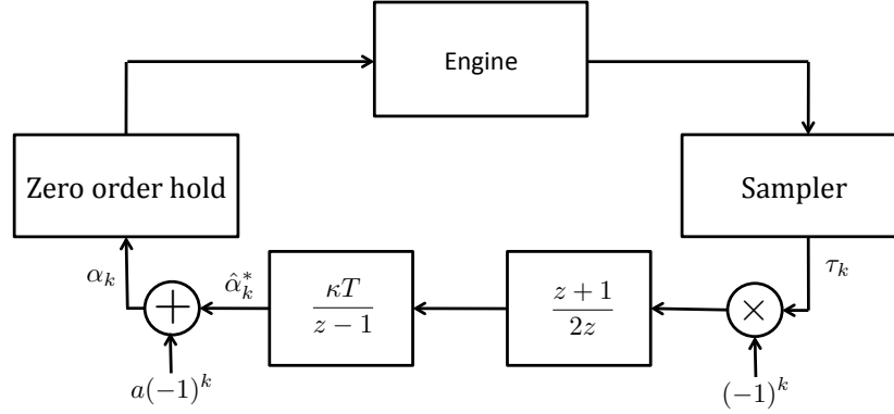
Fig. 9 Proposed sampled data extremum seeking approach for optimal spark estimation on CNG engine
