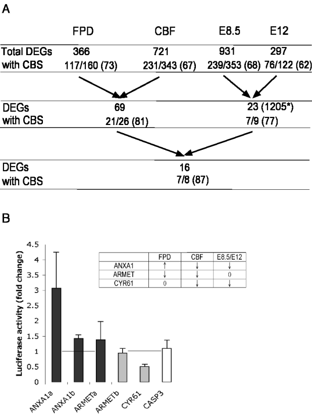
Figure 6 A. Overlaps between the datasets and percentage of genes with a RUNX1 binding site in their regulatory regions. The overlaps between the different platforms are represented with arrows. * indicates that the genes differentially expressed in at least one of the mouse datasets are considered for the following overlap. The number of differentially expressed genes (DEGs) containing a conserved RUNX1 binding site (with CBS) in their regulatory regions, as determined by the oPOSSUM program [27], over the number of analyzed genes is indicated for each dataset and overlap. The corresponding percentage is indicated in brackets. B. Luciferase assay for 5 RUNX1 binding sites corresponding to 3 differentially expressed genes. The transactivation activity of RUNX1 over these sites was measured as the fold change of the luciferase activity in the presence of the CBF complex compared to the endogenous activity of each construct. The standard errors of three independent replicates are shown. CASP3 was shown as a negative control as no binding site was found for this gene. The difference in expression for the three genes in each dataset is indicated in the table. 0 means no difference in expression, ↓ stands for down-regulated and ↑ stands for up-regulated.
