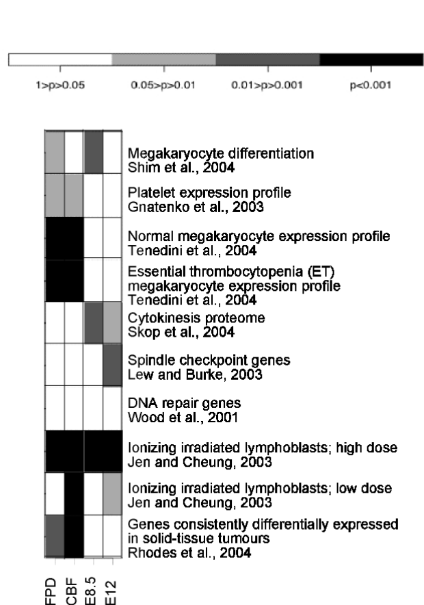
Figure 4 MR-GSE test. Representation of the p-values (corrected for multiple testing) resulting from the MR-GSE test for each dataset and 10 gene sets specified in Additional File 1 (Table S4). In brief they are gene sets Megakaryocyte differentiation, Identification of genes involved in the differentiation of megakaryocytes, DEGs between stem cells and differentiated megakaryocytes; Platelets, Transcription profiling of human blood platelet; ; Normal megakaryocytes, Genes highly expressed in megakaryocytes; ET megakaryocytes, Genes highly expressed in essential thrombocytopenia megakaryocytes; Cytokinesis proteome, Identification of proteins present in the midbody during cytokinesis; Spindle checkpoint, Review; DNA repair, Review; Lymphoblast irradiation; high dose, Effect of ionising radiation on lymphoblasts; Lymphoblast irradiation; low dose, Effect of ionising radiation on lymphoblasts; Genes DE in cancer, Meta-analysis of cancer microarray data to identify genes consistently DE in tumours. This represents whether the genes present in the published gene sets are also differentially expressed in our expression profiles. For example, the genes expressed in normal or diseased megakaryocytes (lines 3 and 4) are significantly represented in the differentially expressed genes identified in the FPD and CBF approaches.
