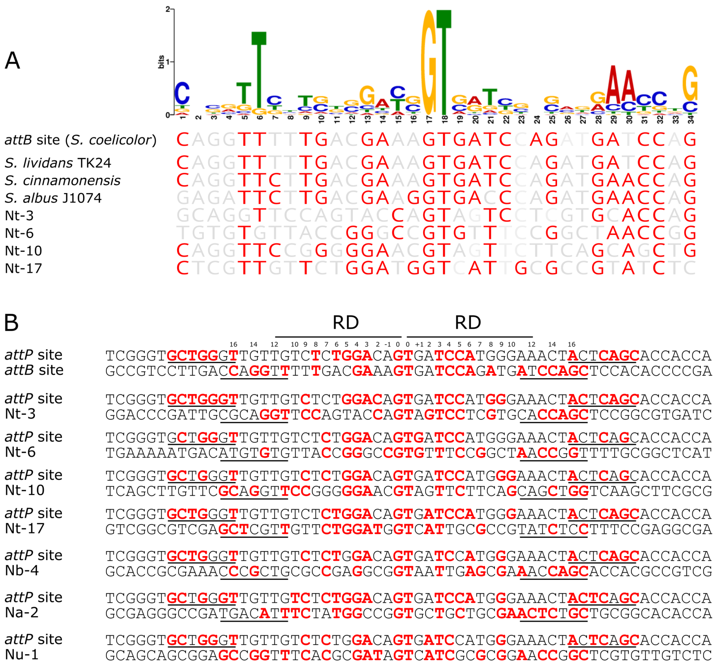
Figure 4 The pseudo- attB motif in Nocardia species and comparison of pseudo- attB sites with attP . (A) Alignment of attB sites with the pseudo- attB motif identified from Nocardia pseudo- attB insertion sites. Red nucleotides are those that are identical to the most common nucleotide at each position within the predicted motif. (B) Alignment of \Phi BT1 attP and attB sites. The canonical attP – attB sites from \Phi BT1 and S. coelicolor , respectively, are shown at the top, followed by an alignment of attP with the most common N. terpenica pseudo- attB sites, as well as those pseudo- attB sites that were most commonly seen from the other Nocardia species investigated in this study. The four predicted ZD binding motifs for \Phi BT1 Int on each attP and pseudo- attB half site are underlined, with the predicted RD binding site shown at the top. Residues that are identical in three of the four ZD motifs within each alignment are shown in red. Residues that are identical at three out of four positions within -/+10 of the RD binding region are also shown in red. The central GT dinucleotide is in red and labelled as position 0.
