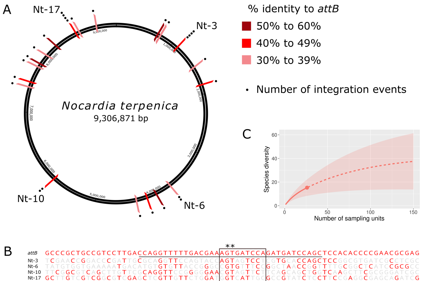
Figure 2 Pseudo- attB insertion sites in N. terpenica AUSMD00012715. (A) Locations of individual pRT801 insertion sites mapped onto the N. terpenica AUSMDU00012715 genome. Percentage similarity to the minimal attB site of S. coelicolor is indicated by varying shades of red. (B) Comparison of the most common N. terpenica pseudo- attB sites with the 73b canonical attB sequence from S. coelicolor (a comparison of all sites can be found in Fig. S1). Red nucleotides indicate identity to the canonical attB sequence. The common attB – attP core is boxed and the minimal attB sequence is underlined. The core GT dinucleotide is denoted by asterisks. (C) Rarefaction analysis showing number of predicted sites in the N. terpenica AUSMDU00012715 genome.
