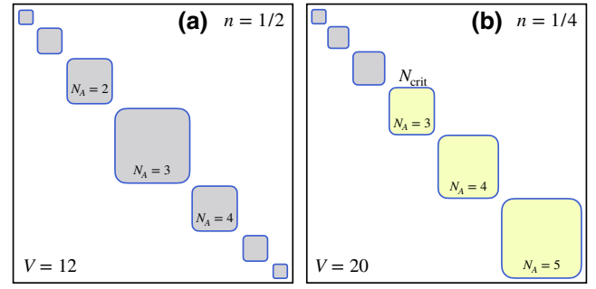
FIG. 4. Sketch of the block dimensions of the reduced density matrix \hat{\rho}_A of subsystem A at the subsystem fraction f = \frac{1}{2} . (a) Case V=12 at half filling n = \frac{1}{2} , for which V_A = 6 . The number of particles ranges from N_A = 0 to N_A = 6 , with N_A = 3 representing the largest block. (b) Case V=20 at quarter filling n = \frac{1}{4} , for which V_A = 10 . The number of particles ranges from N_A = 0 to N_A = 5 , with N_A = 5 representing the largest block. The blocks with N_A \geq N_{\text{crit}} = 3 are larger than the corresponding blocks in subsystem B (not shown in the figure).
