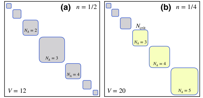
FIG. 4. Sketch of the block dimensions of the reduced density matrix \hat{\rho}_A of subsystem A at the subsystem fraction f = \frac{1}{2} . (a) Case V = 12 at half filling n = \frac{1}{2} , for which V_A = 6 . The number of particles ranges from N_A = 0 to N_A = 6 , with N_A = 3 representing the largest block. (b) Case V = 20 at quarter filling n = \frac{1}{4} , for which V_A = 10 . The number of particles ranges from N_A = 0 to N_A = 5 , with N_A = 5 representing the largest block. The blocks with N_A \geq N_{\text{crit}} = 3 are larger than the corresponding blocks in subsystem B (not shown in the figure).
