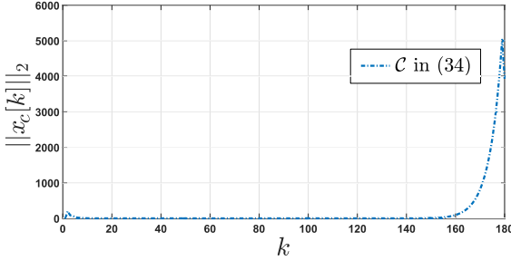
Fig. 4. Norm of the state of the quantized controller \|x_c[k]\|_2 in (36) with quantizer resolution (n, m) = (24, 14) .
