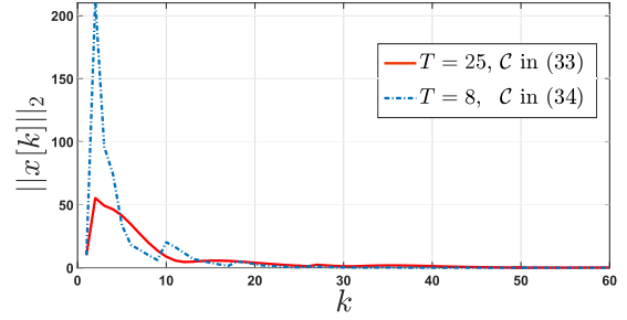
Fig. 1. Norm of the state of the closed-loop system \|x[k]\|_2 with quantized controller (25) and quantizer resolution (n, m) = (24, 14) .
