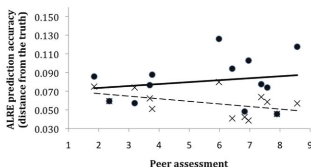
Figure 2. Peer assessment of expert knowledge versus actual performance for the participants in Workshop 3. Prediction accuracy is calculated as ALRE (see text). Small values for prediction accuracy are better. Closed circles and the solid line are estimates from round 1 ( r=0.19 ). Crosses and the dashed line are estimates from round 2 ( r=-0.47 ). Estimates closer to the x-axis indicate the answers are closer to the truth.
