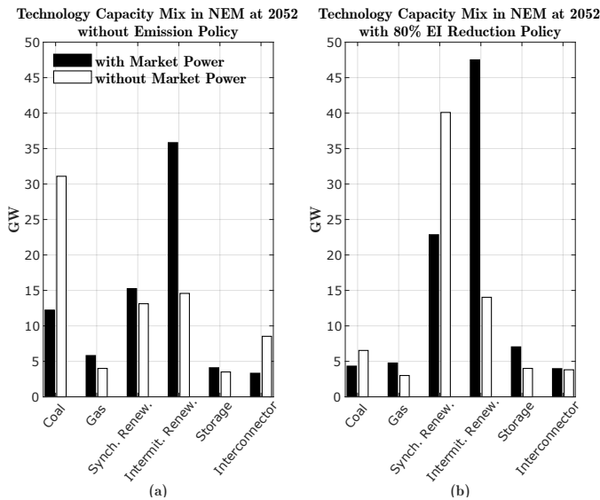
Fig. 6: Technology capacity mix in NEM with and without considering market power for (a) No Emission Reduction policy, (b) 80% Emission Intensity Reduction policy.
