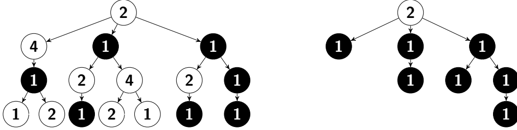
Figure 4.4: A realisation of \{\bar{\mathbf{Z}}_n^{(4)}\} (left) with the corresponding realisation of the \{\mathbf{Z}_n^{(e,4)}\} (right) when \boldsymbol{\alpha}^{(k)} = \mathbf{e}_1 . The black nodes represent individuals with type greater than 4 which are immediately replaced with type 1.
