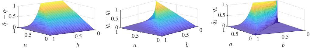
Figure 4.2: Differences in the extinction probabilities related to Example 1, plotted as a function of the parameters a and b .
