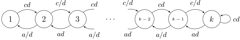
Figure 6.1: The mean progeny representation graph corresponding to \{\bar{\mathbf{Z}}_n^{(k)}\} when k is odd in Example 2.
