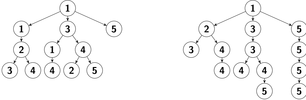
Figure 4.3: A realisation of \{\mathbf{Z}_n\} (left). The corresponding seed process, as introduced in Definition 1, is \mathbf{S}_0 = (1, 0, 0, \dots) , \mathbf{S}_1 = (0, 1, 1, 0, 1, \dots) , \mathbf{S}_2 = (0, 0, 2, 1, 1, \dots) , \mathbf{S}_3 = (0, 0, 0, 3, 1, \dots) , \mathbf{S}_4 = (0, 0, 0, 0, 2, \dots) and \mathbf{S}_5 = (0, 0, 0, 0, 0, \dots) . The right graph illustrates the tree representation of \{\mathbf{S}_k\} .
