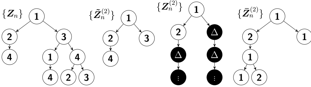
Figure 3.1: A visualisation of \{\mathbf{Z}_n\} , \{\tilde{\mathbf{Z}}_n^{(2)}\} , \{\mathbf{Z}_n^{(2)}\} and \{\bar{\mathbf{Z}}_n^{(2)}\} corresponding to a specific realisation \omega \in \Omega . It is such that \mathbf{r}_{\langle 0 \rangle} = \mathbf{e}_2 + \mathbf{e}_3 , \mathbf{r}_{\langle 12 \rangle} = \mathbf{e}_4 , \mathbf{r}_{\langle 13 \rangle} = \mathbf{e}_1 + \mathbf{e}_4 , \mathbf{r}_{\langle 1311 \rangle} = \mathbf{e}_4 , \mathbf{r}_{\langle 1314 \rangle} = \mathbf{e}_2 + \mathbf{e}_3 and \mathbf{r}_{\langle 1214 \rangle} = \mathbf{r}_{\langle 131114 \rangle} = \mathbf{r}_{\langle 131412 \rangle} = \mathbf{r}_{\langle 131413 \rangle} = \mathbf{0} are used to construct \{\mathbf{Z}_n\} , \{\tilde{\mathbf{Z}}_n^{(2)}\} and \{\mathbf{Z}_n^{(2)}\} , and additionally X_1^{(2)}(\omega, \langle 0 \rangle) = 1 , \mathbf{r}_{\langle 11 \rangle} = \mathbf{0} , X_1^{(2)}(\omega, \langle 12 \rangle) = 1 , \mathbf{r}_{\langle 1211 \rangle} = \mathbf{e}_1 + \mathbf{e}_2 and \mathbf{r}_{\langle 121111 \rangle} = \mathbf{r}_{\langle 121112 \rangle} = \mathbf{0} are used to construct \{\bar{\mathbf{Z}}_n^{(k)}\} . All other information contained in \omega is not required.
