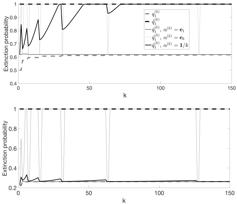
Figure 6.4: Sequences of extinction probabilities \tilde{q}_1^{(k)} , q_1^{(k)} and \bar{q}_1^{(k)} for different replacement distributions and different parameters values, corresponding to Example 3. Details are given in the text.
