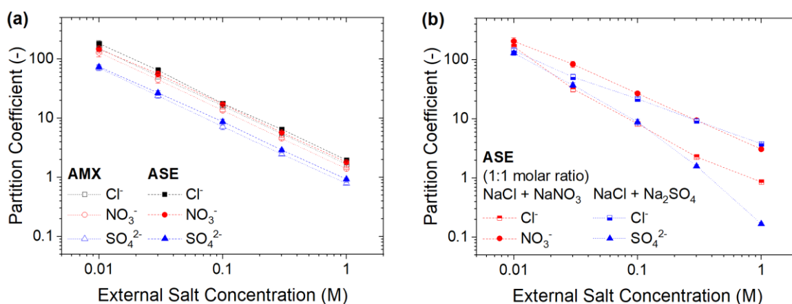
Figure 9. Partition coefficient of counter-ions in anion exchange membranes for (a) single salt experiments in AMX and ASE where \text{NaCl} , \text{NaNO}_3 and \text{Na}_2\text{SO}_4 were used in external solutions and for (b) binary salts experiments in ASE where equimolar mixtures of \text{NaCl} + \text{NaNO}_3 and \text{NaCl} + \text{Na}_2\text{SO}_4 were used in external solutions.
