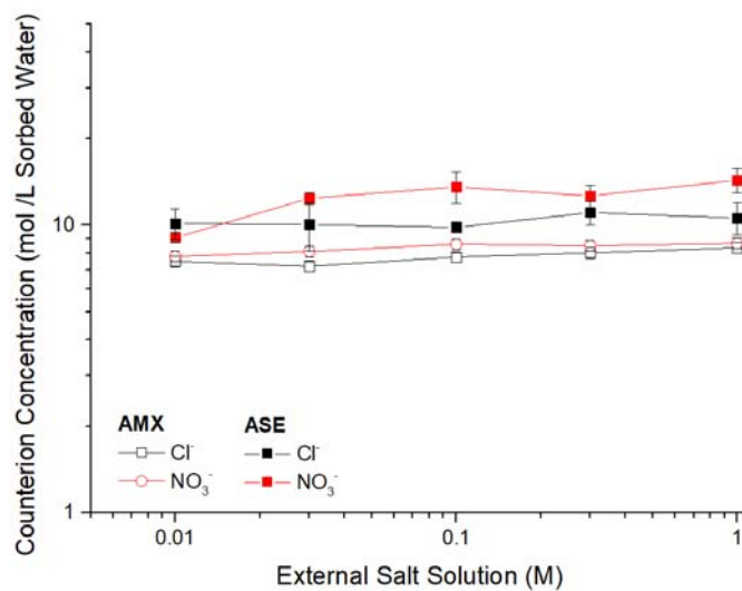
Figure S1 Counter-ion concentration (mol/L sorbed water) of chloride and nitrate in AMX and ASE, equilibrated in single salt solutions with sodium as the co-ion.
