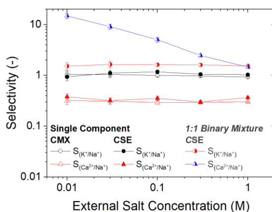
Figure 7. Selectivity of \text{K}^+ and \text{Ca}^{2+} to \text{Na}^+ in cation exchange membranes for single salt experiments in CMX and CSE where \text{NaCl} , \text{KCl} and \text{CaCl}_2 were used in external solutions; and for binary salts
