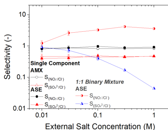
Figure 10. Selectivity of NO_3^- and SO_4^{2-} to Cl^- for single salt experiments in AMX and ASE where NaCl, NaNO_3 and Na_2SO_4 were used in external solutions; and for binary salts experiments in ASE where equimolar mixtures of NaCl + NaNO_3 and NaCl + Na_2SO_4 were used in external solutions.
