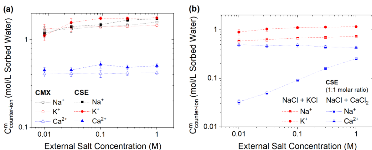
Figure 5. Counter-ion concentration for (a) single salt experiments in cation exchange membranes CMX and CSE, where NaCl, KCl and \text{CaCl}_2 were used in external solutions, and for (b) binary salts experiments in CSE where equimolar mixtures of NaCl + KCl and NaCl + \text{CaCl}_2 were used in external solutions. Lines are drawn to guide the eye.
