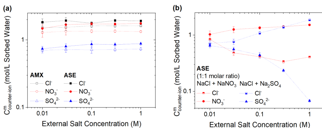
Figure 8. Counter-ion concentration in anion exchange membranes for (a) single salt experiments in AMX and ASE where NaCl, NaNO 3 and Na 2 SO 4 were used in external solutions and for (b) binary salts experiments in ASE where equimolar mixtures of NaCl + NaNO 3 and NaCl + Na 2 SO 4 were used in external solutions.
