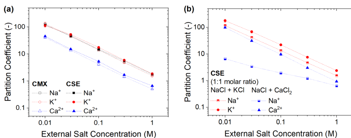
Figure 6. Partition coefficient of counter-ions in cation exchange membranes for (a) single salt experiments in CMX and CSE where \text{NaCl} , \text{KCl} and \text{CaCl}_2 were used in external solutions and for (b) binary salts experiments in CSE where equimolar mixtures of \text{NaCl} + \text{KCl} and \text{NaCl} + \text{CaCl}_2 were used in external solutions.
