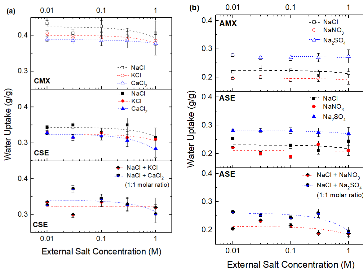
Figure 1. Water uptake of (a) cation exchange membranes (CMX and CSE) and (b) anion exchange membranes (AMX and ASE) after equilibration in different external salt solutions of concentrations ranging from 0.01 M to 1 M. Equimolar binary mixtures of NaCl + KCl and NaCl + CaCl 2 were used for CSE membranes (a), and those of NaCl + NaNO 3 and NaCl + Na 2 SO 4 were used for ASE membranes (b). The dashed lines are drawn to guide the eye.
