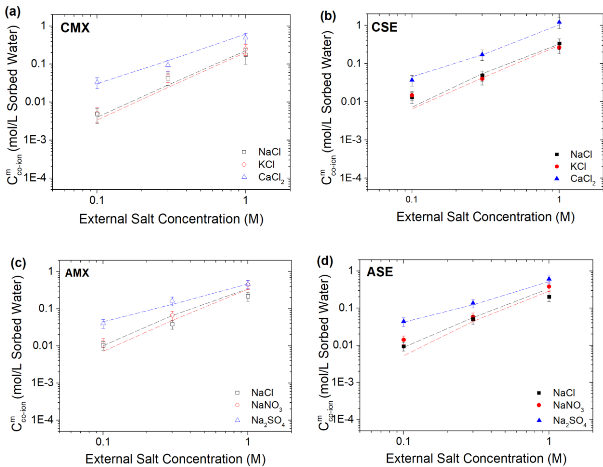
Figure 2. Concentration of co-ion (expressed in mol/L sorbed water)) in cation exchange membranes (i.e., [Cl - ] in CEM (a) and CSE (b)) and anion exchange membranes (i.e., [Na + ] in AMX (c) and ASE (d)) as a function of external salt concentration. Data are shown for single salts experiments, and are fitted to Eq. (6) for MX salts in IEMs, and Eq. (S1) for CaCl 2 in CEMs and Na 2 SO 4 in AEMs. The fitting was performed using all three sets of data for each membrane, treating \xi as the only fitting parameter ( \xi_{\text{CMX}} = 1.0 \pm 0.1 , \xi_{\text{CSE}} = 2.8 \pm 0.5 , \xi_{\text{AMX}} = 4.8 \pm 1.4 , and \xi_{\text{ASE}} = 5.4 \pm 1.5 ).
